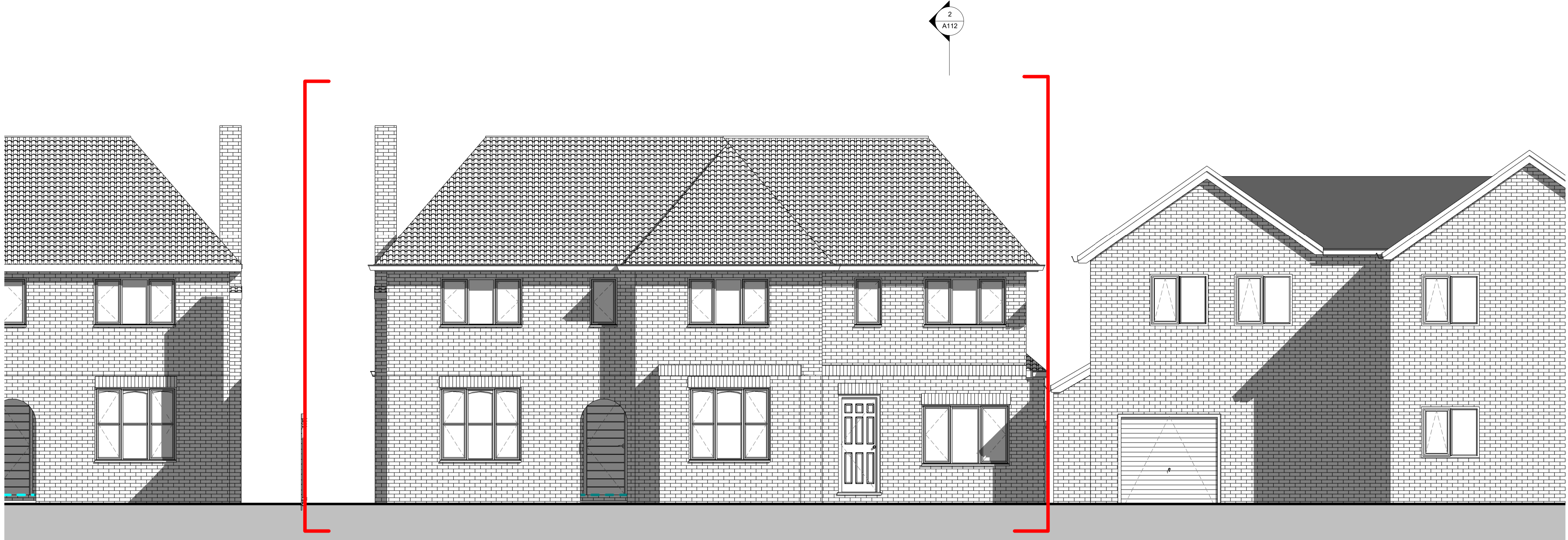
1 Proposed S-W Elevation 1:50
