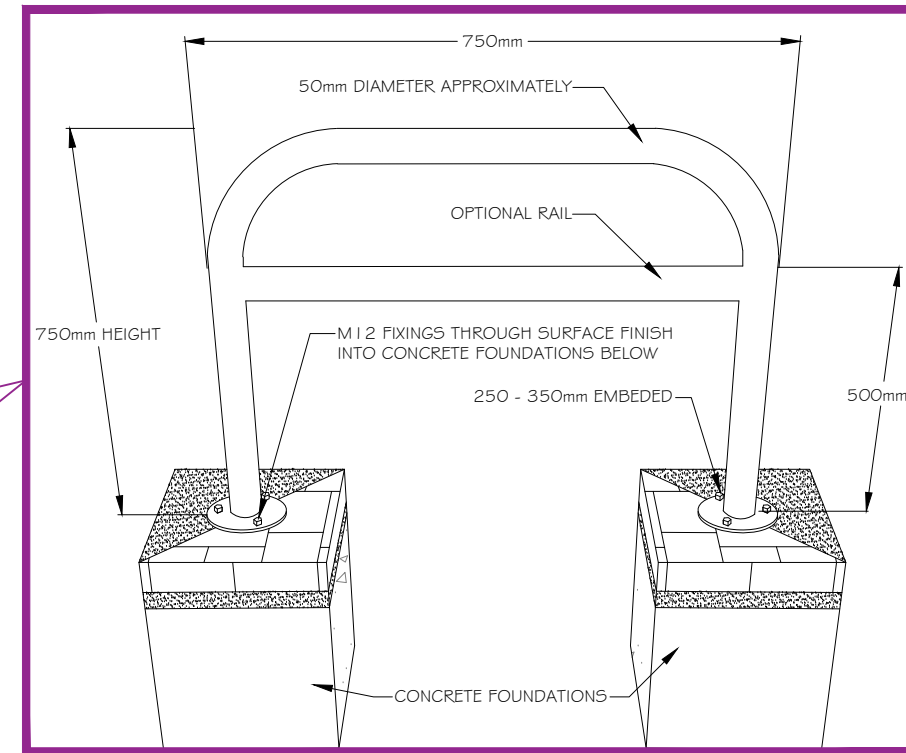
DETAIL OF SHEFFIELD STAND
