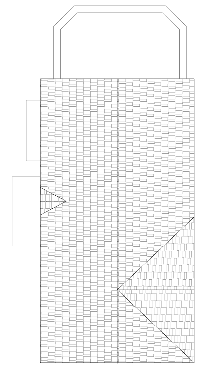
ROOF PLAN
