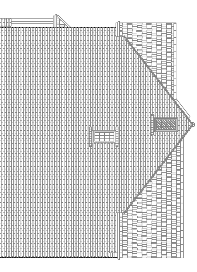
PROPOSED NORTH EAST ELEVATION 1:100
