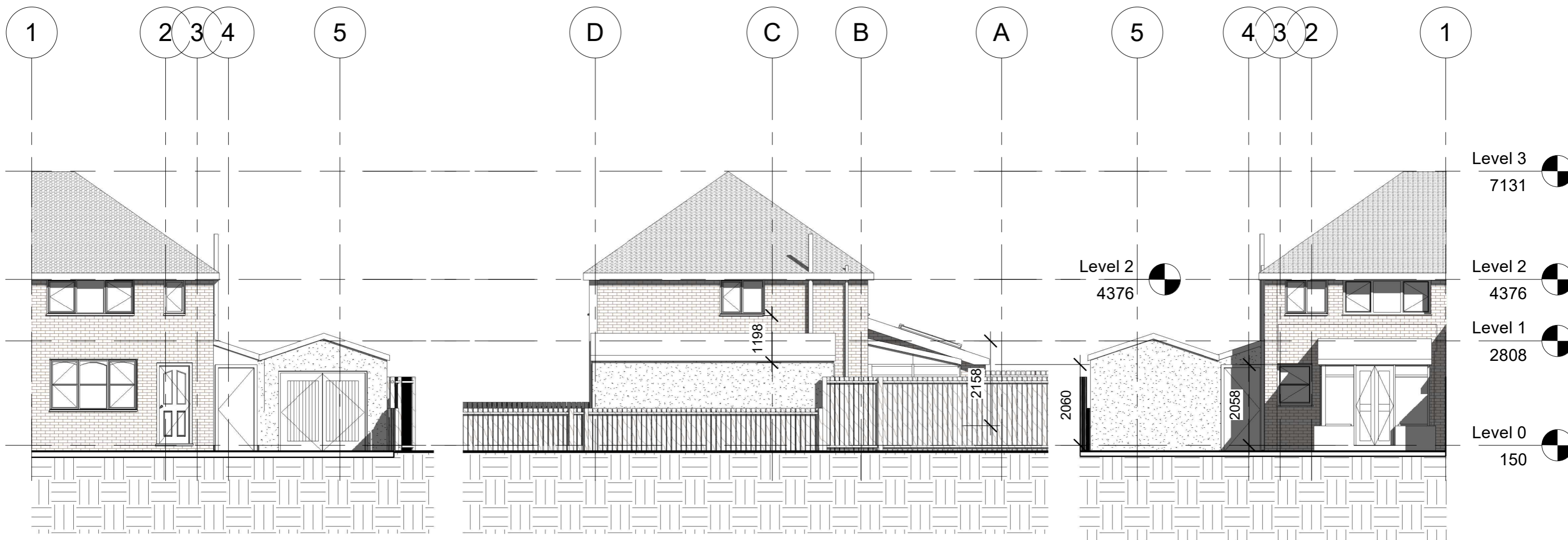
1 Existing front elevation 1 : 100
