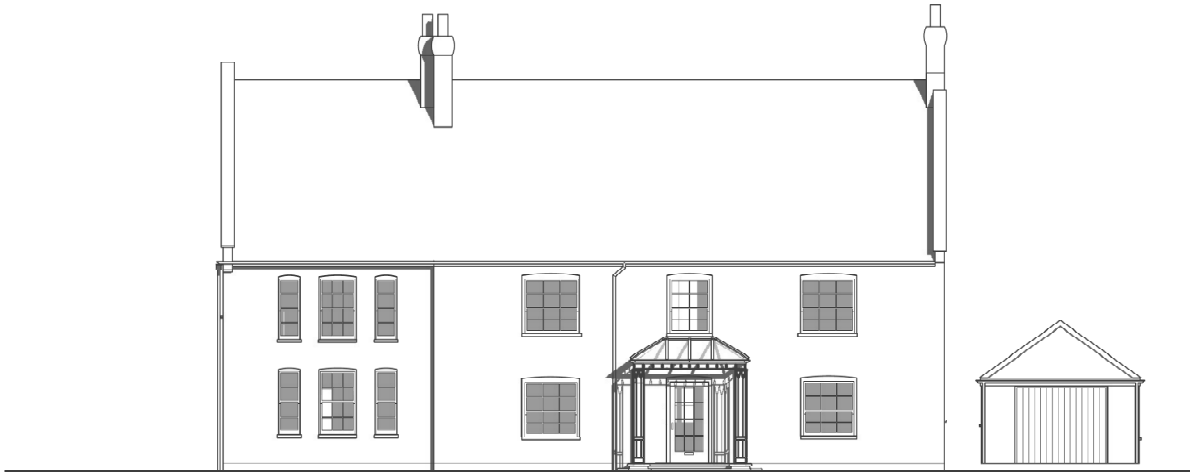
East Elevation
