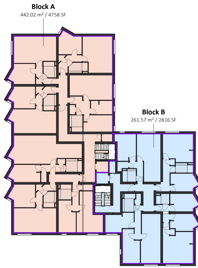
2 GIFA_Plan_01-First 1:300
