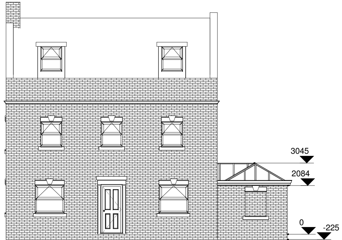
2 Proposed Front Elevation 1 : 100
