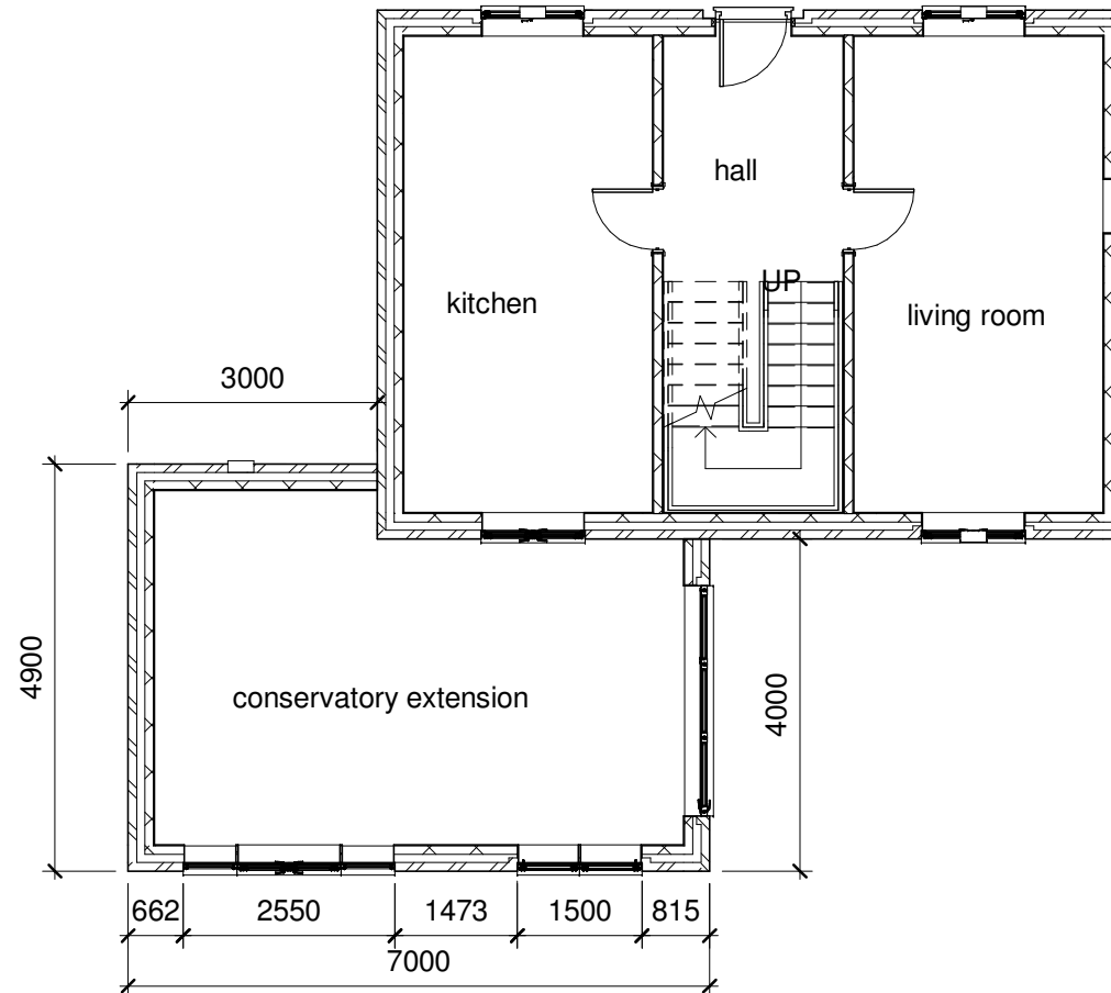
2 Ground Floor Proposed 1 : 100
