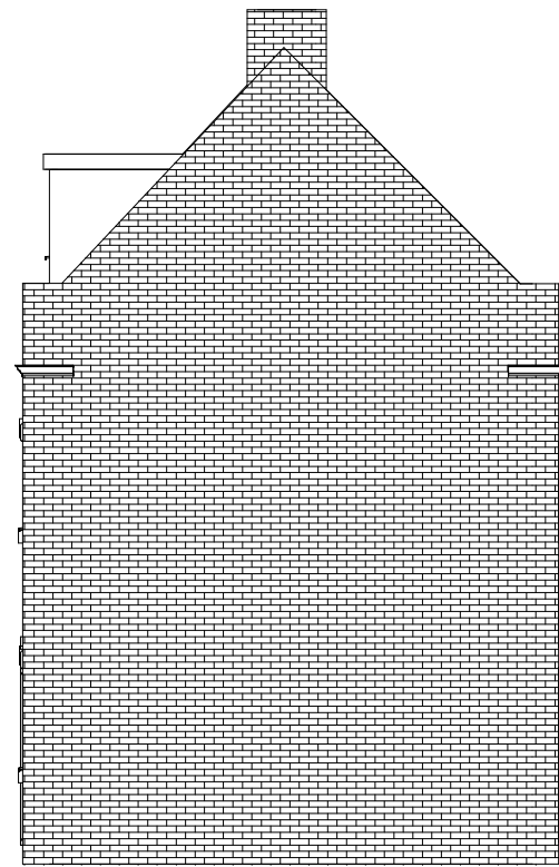
3 Existing Side Elevation 1 : 100
