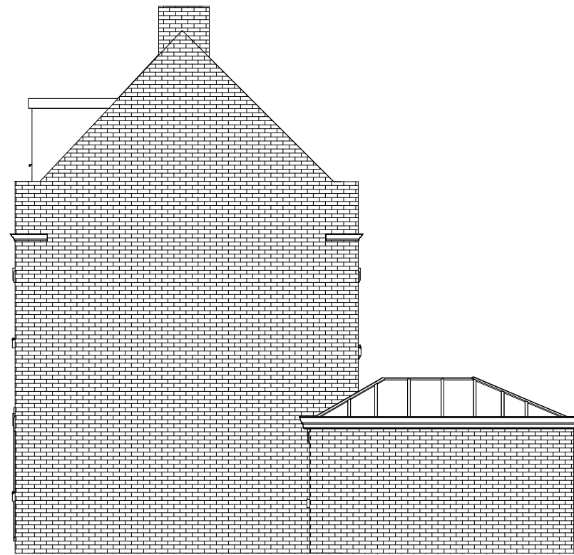
4 Proposed Side Elevation 1 : 100
