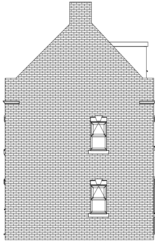
1 Existing Side Elevation 1 : 100
