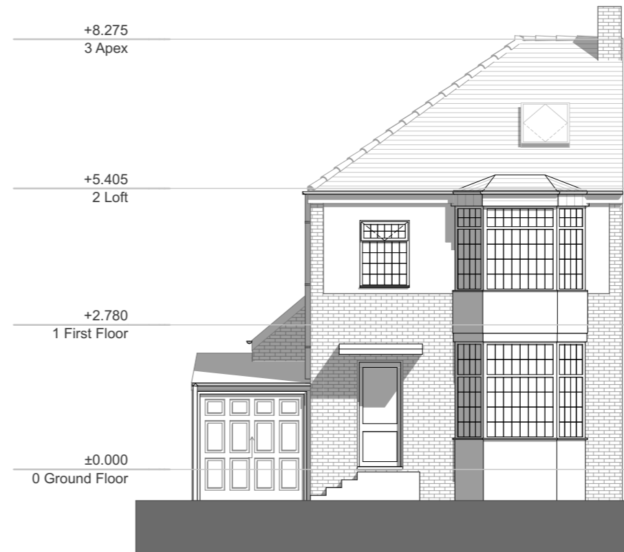
E-01 Existing North West Elevation 1:100
