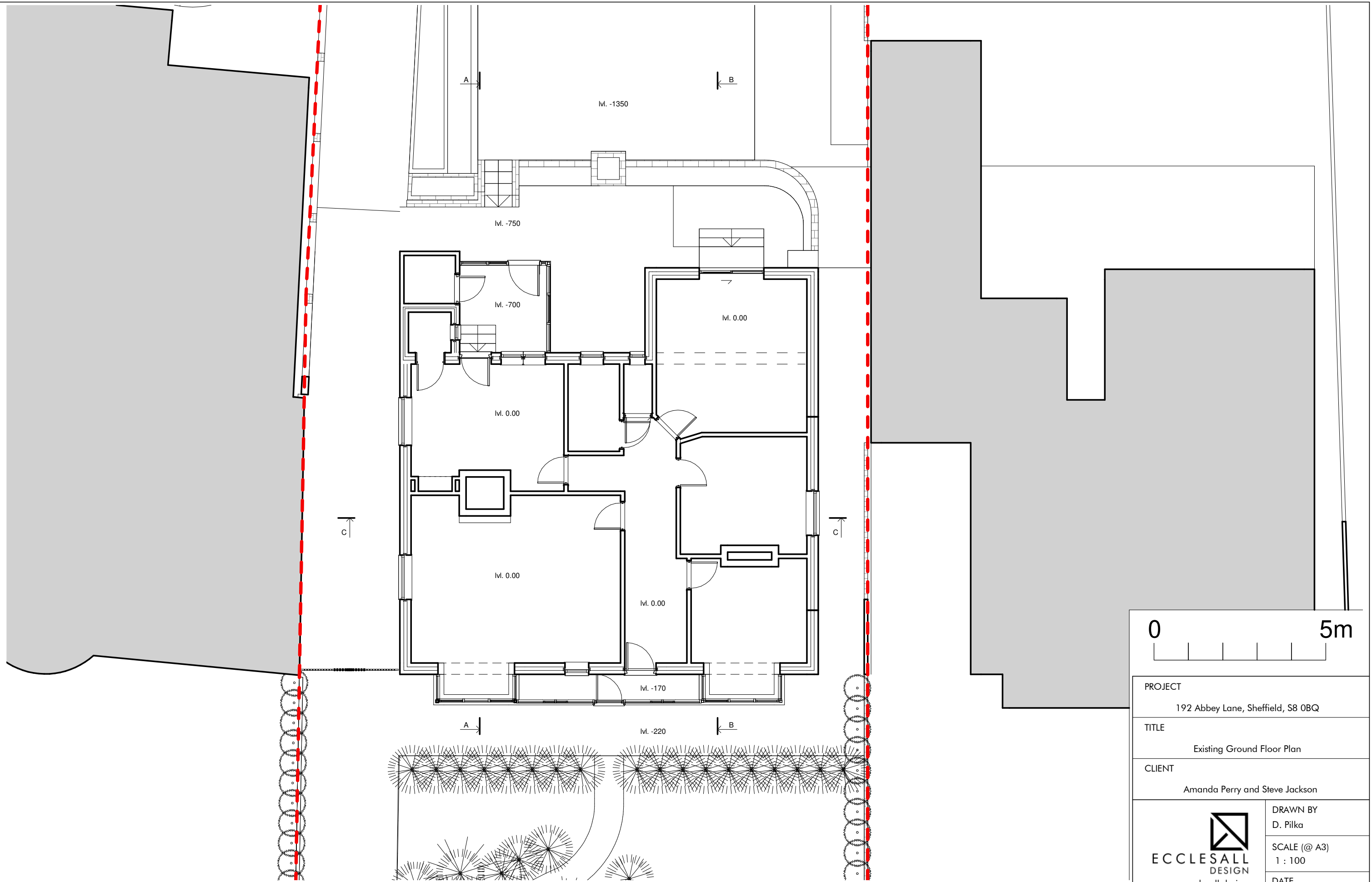
Existing Ground Floor Plan 1 : 100
