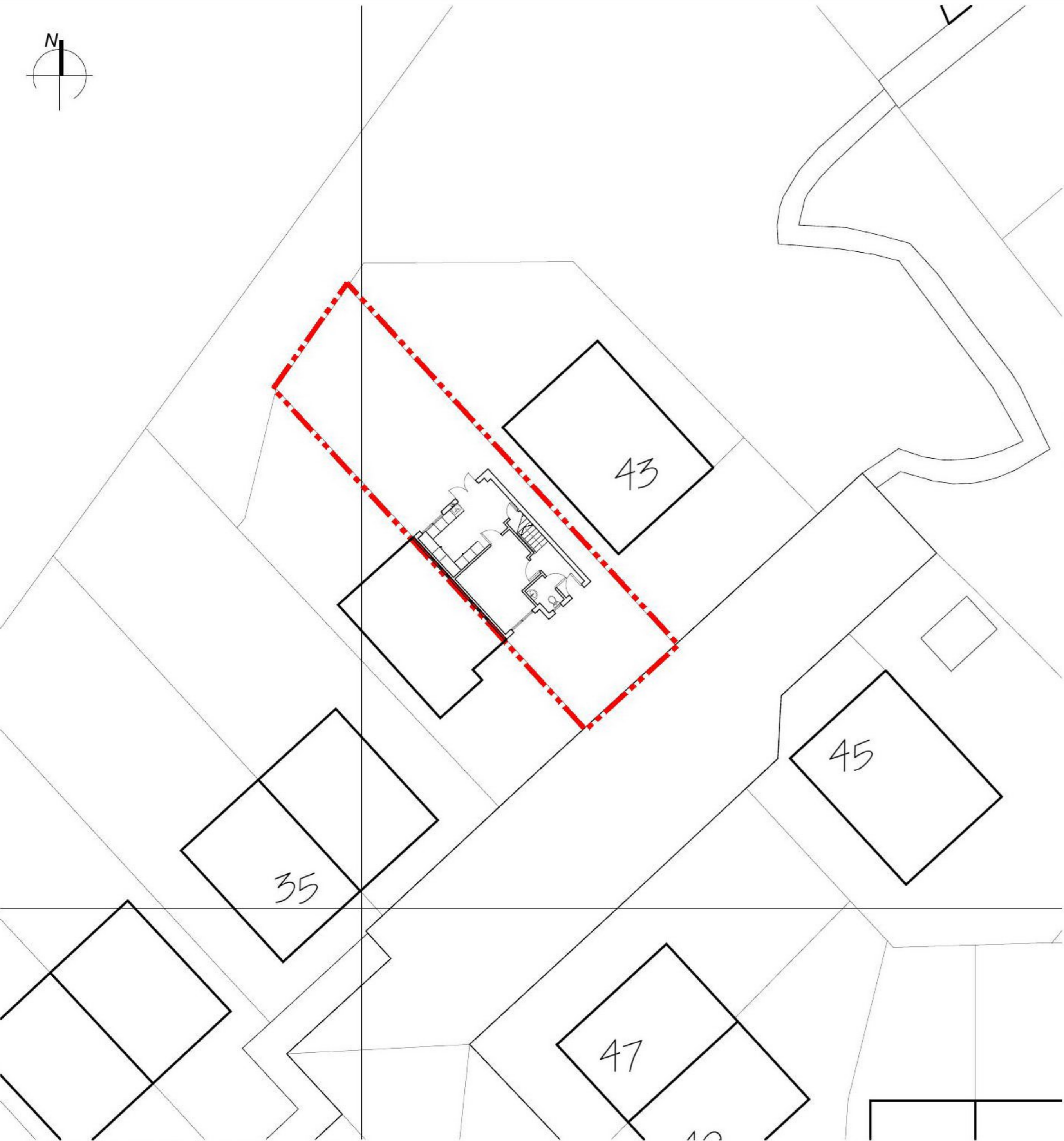
BLOCK PLAN AS EXISTING & PROPOSED @ 1:250
