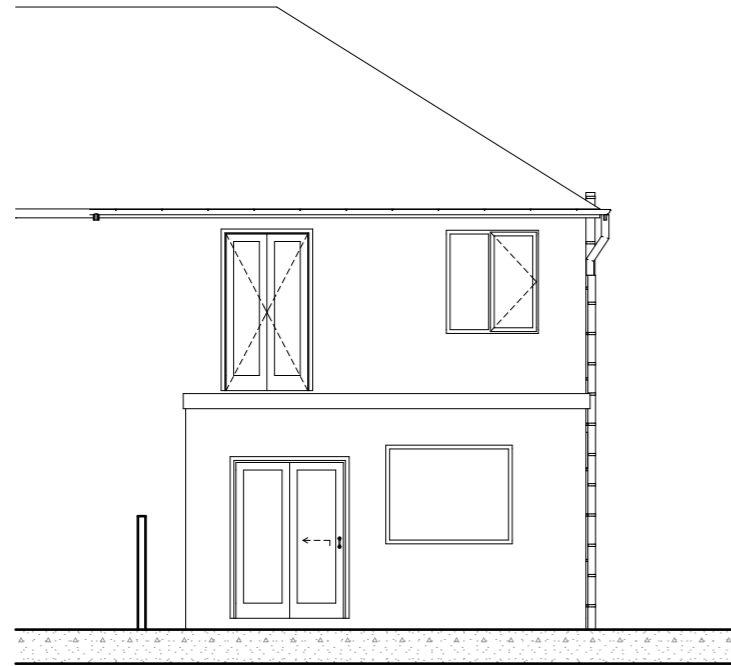
RE3 Rear Elevation 1:100
