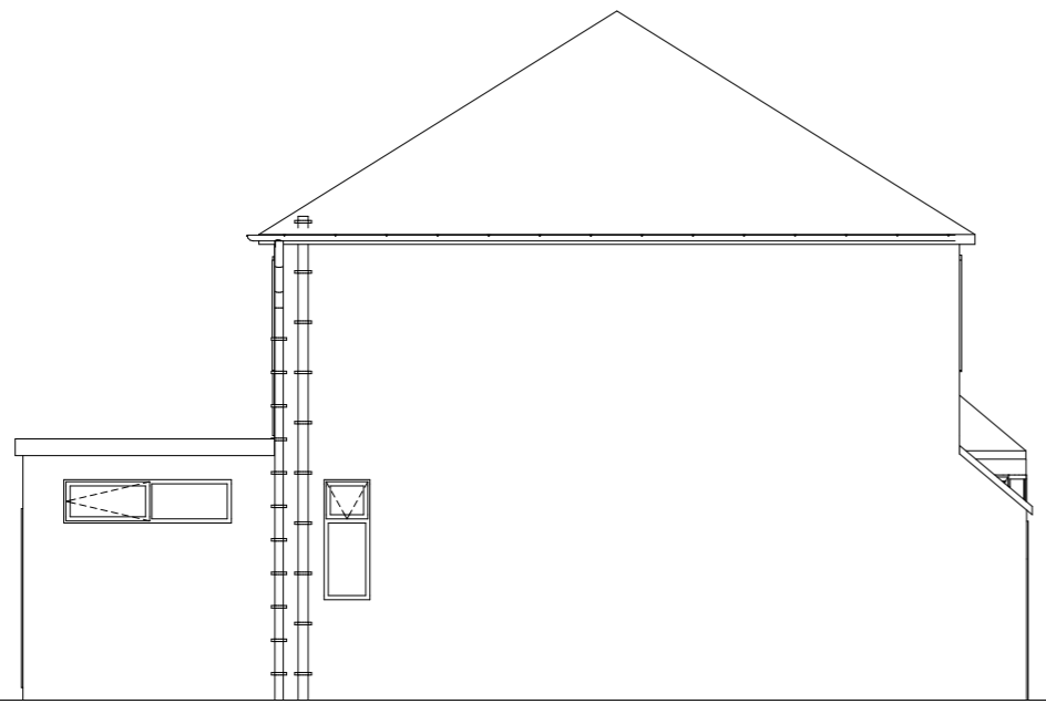
SRE3 Side Right Elevation 1:100
