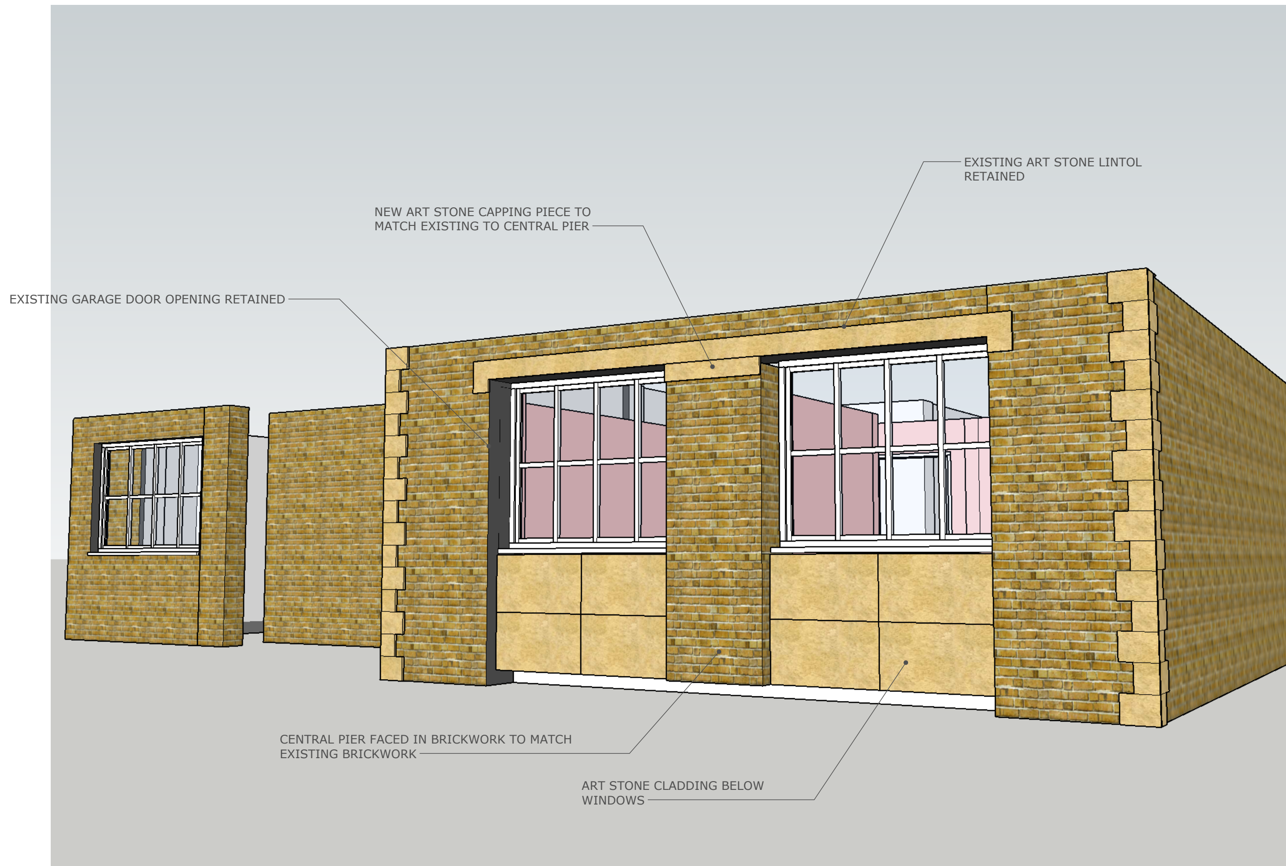
DETAIL OF PROPOSED GARAGE DOOR INFILL - NTS
