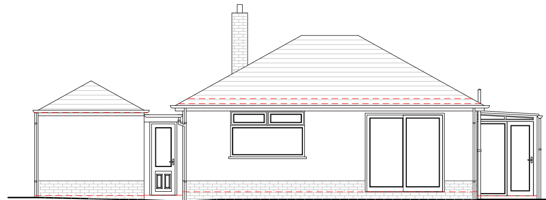
Rear Elevation
