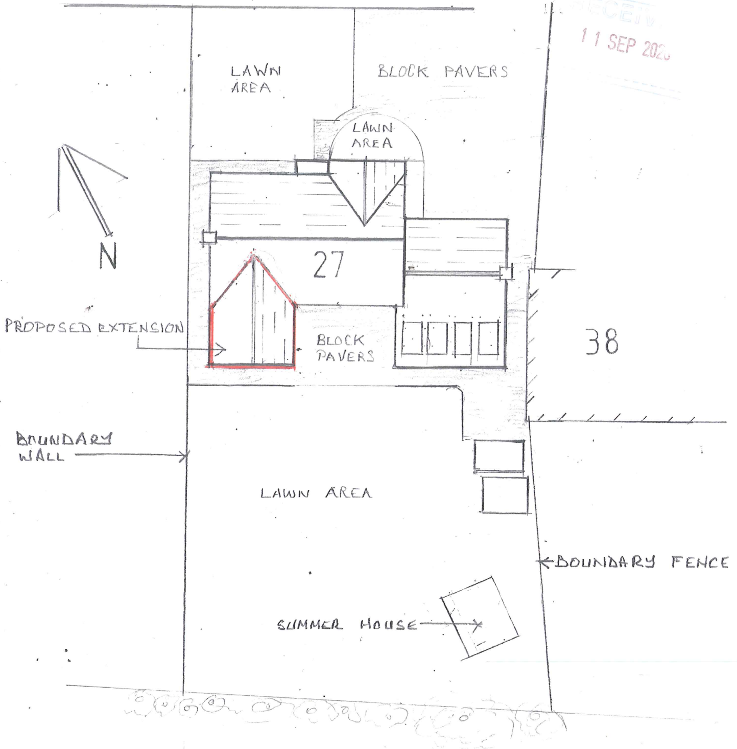
PROPOSED BLOCK PLAN AT 27 BARN CLOSE NEWBOLD SCALE 1 - 200.
