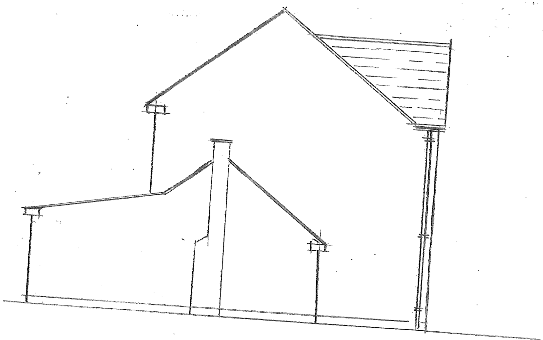
EXTG. SIDE ELEVATION AT 27 BARN CLOSE NEWBOLD SCALE 1-100
