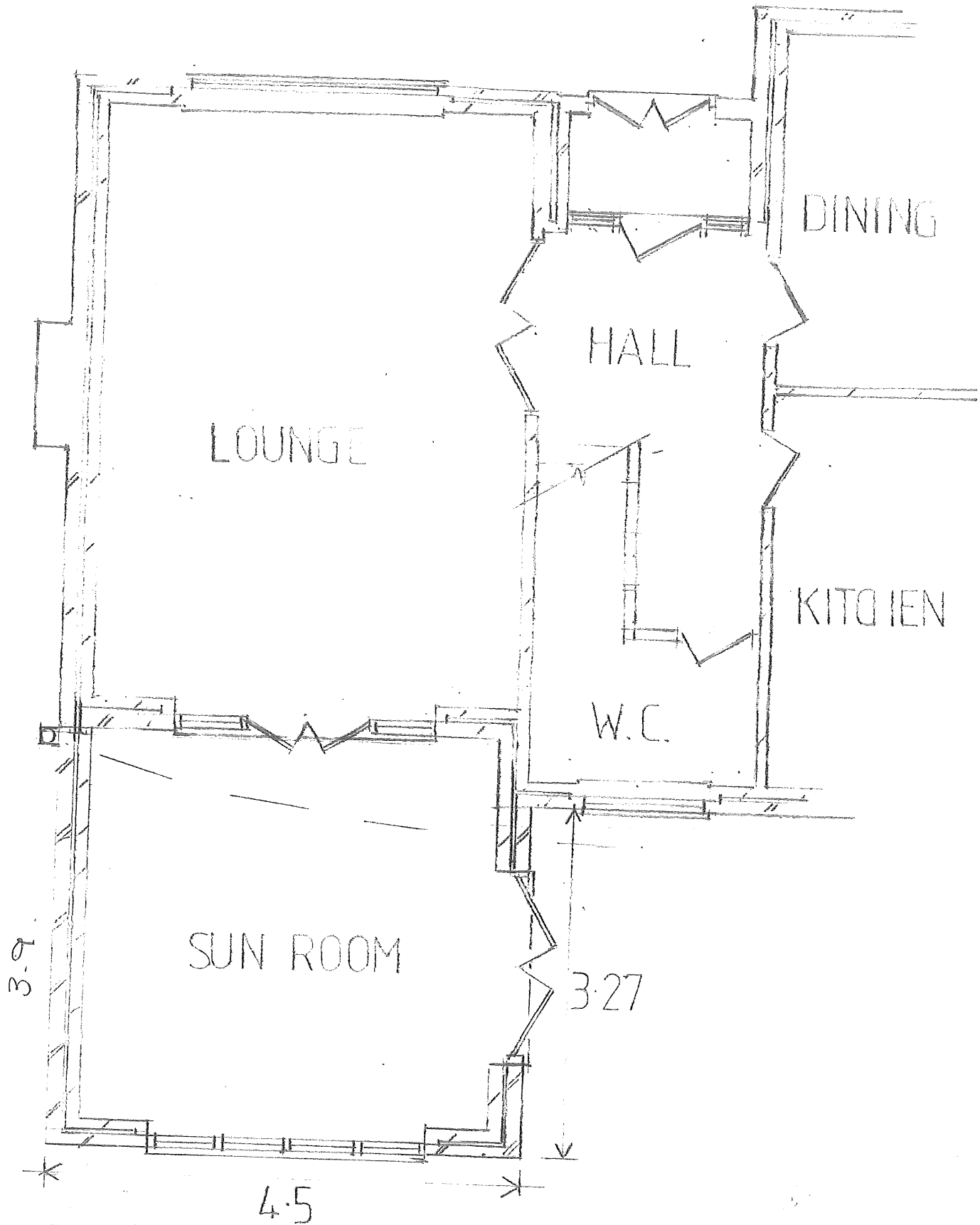
PROPOSED GROUND FLOOR PLAN AT 27 BARN CLOSE NEWBOLD SCALE 1-50
