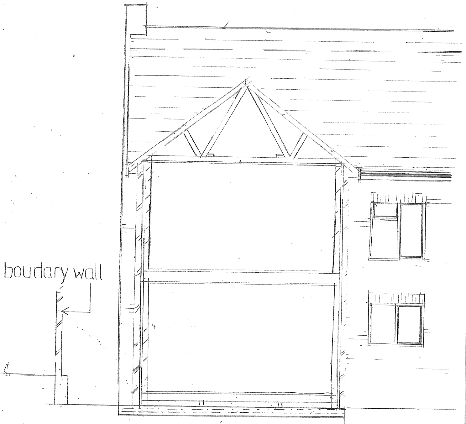
PROPOSED SECTION AT 27 BARN CLOSE NEWBOLD SCALE 1-50
