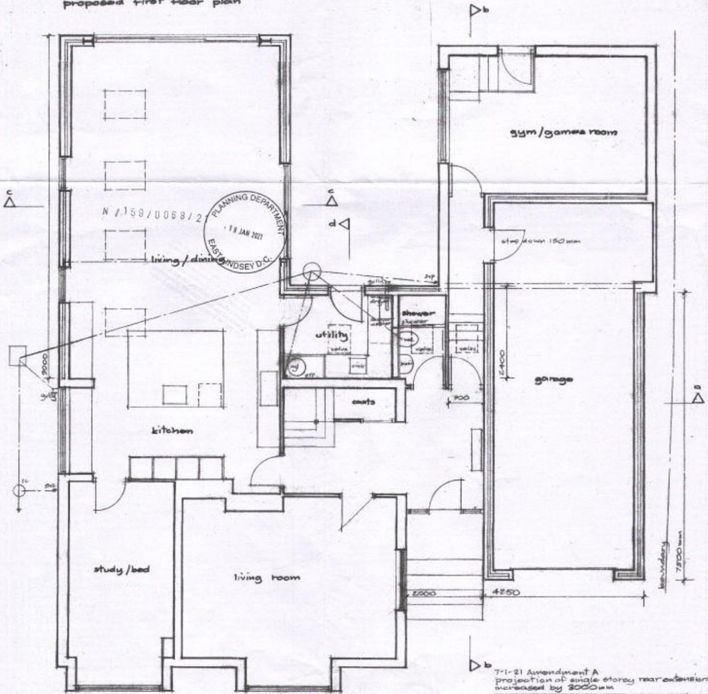
proposed extension & alterations to Oak Lodge, South Elkington, Louth
