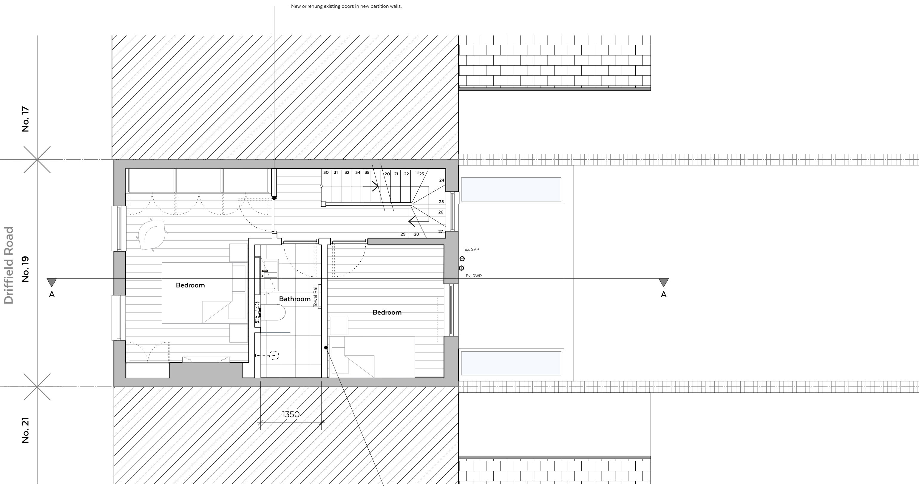
Proposed First Floor Plan - 1:50 @ A3
