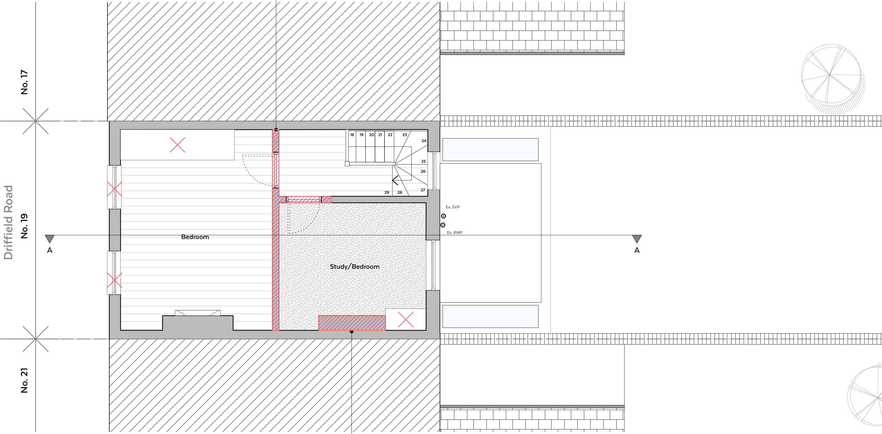
Existing First Floor Plan - 1:50 @ A3
