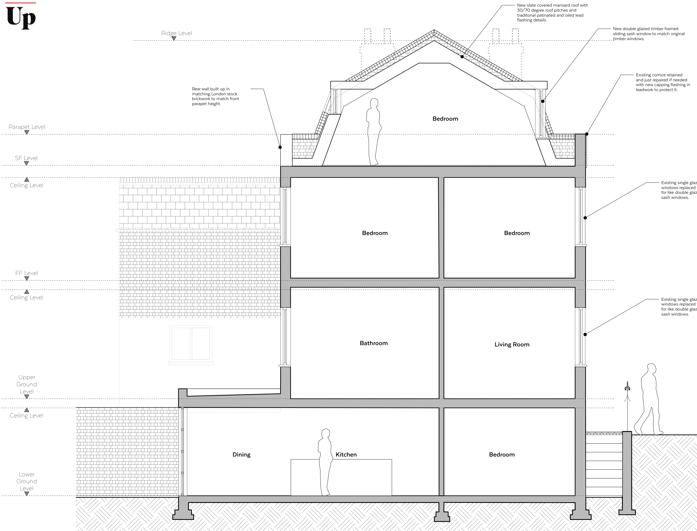
Proposed Section AA - 1:50 @ A3
