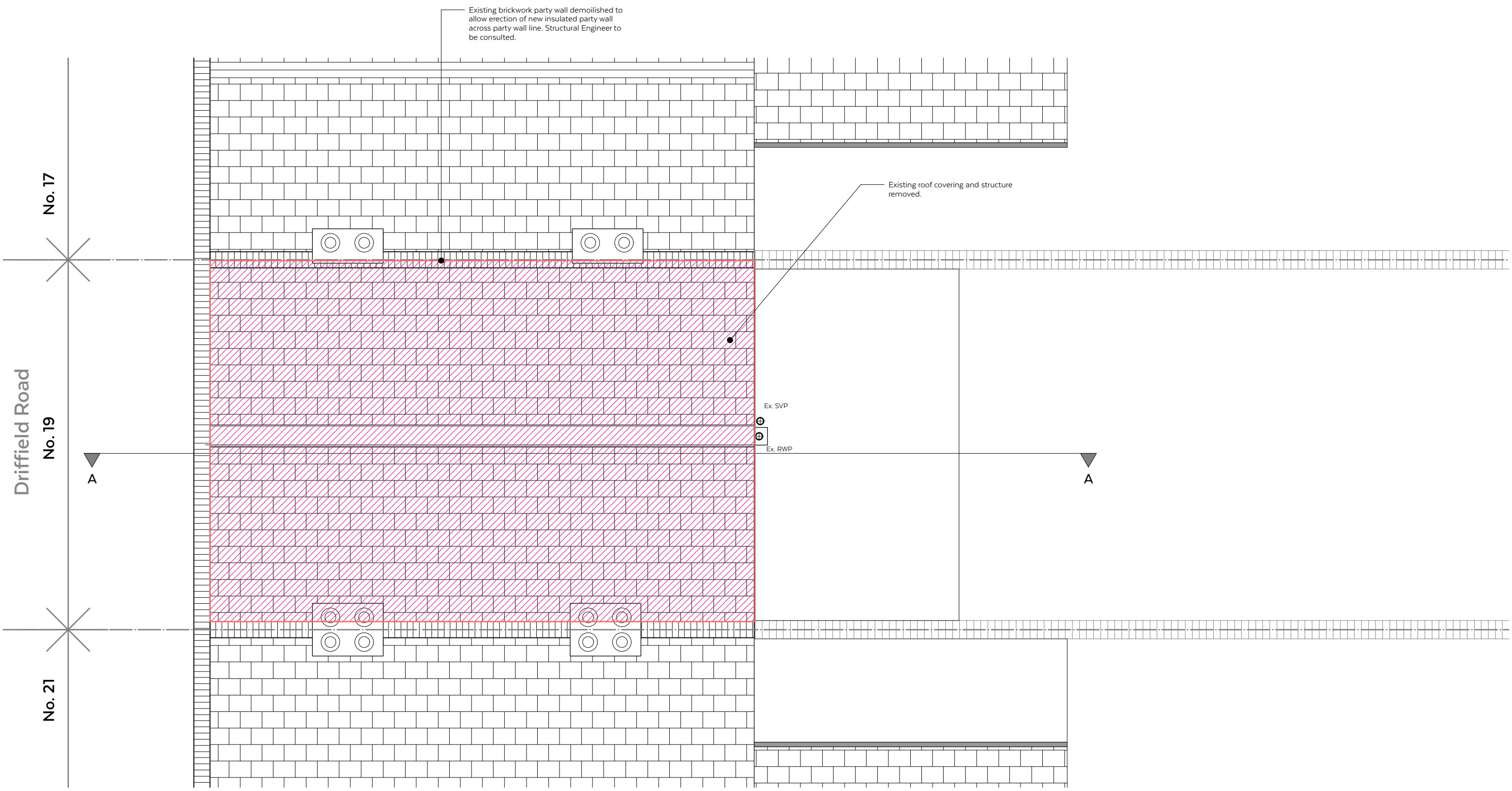
Existing Roof Plan - 1:50 @ A3
