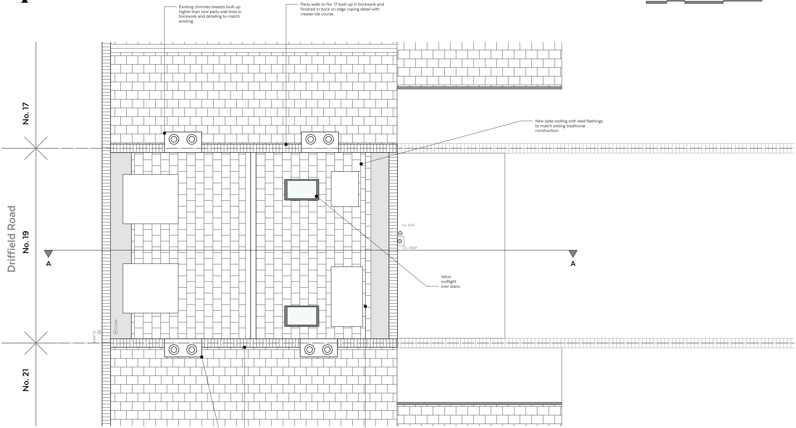
Proposed Roof Plan - 1:50 @ A3
