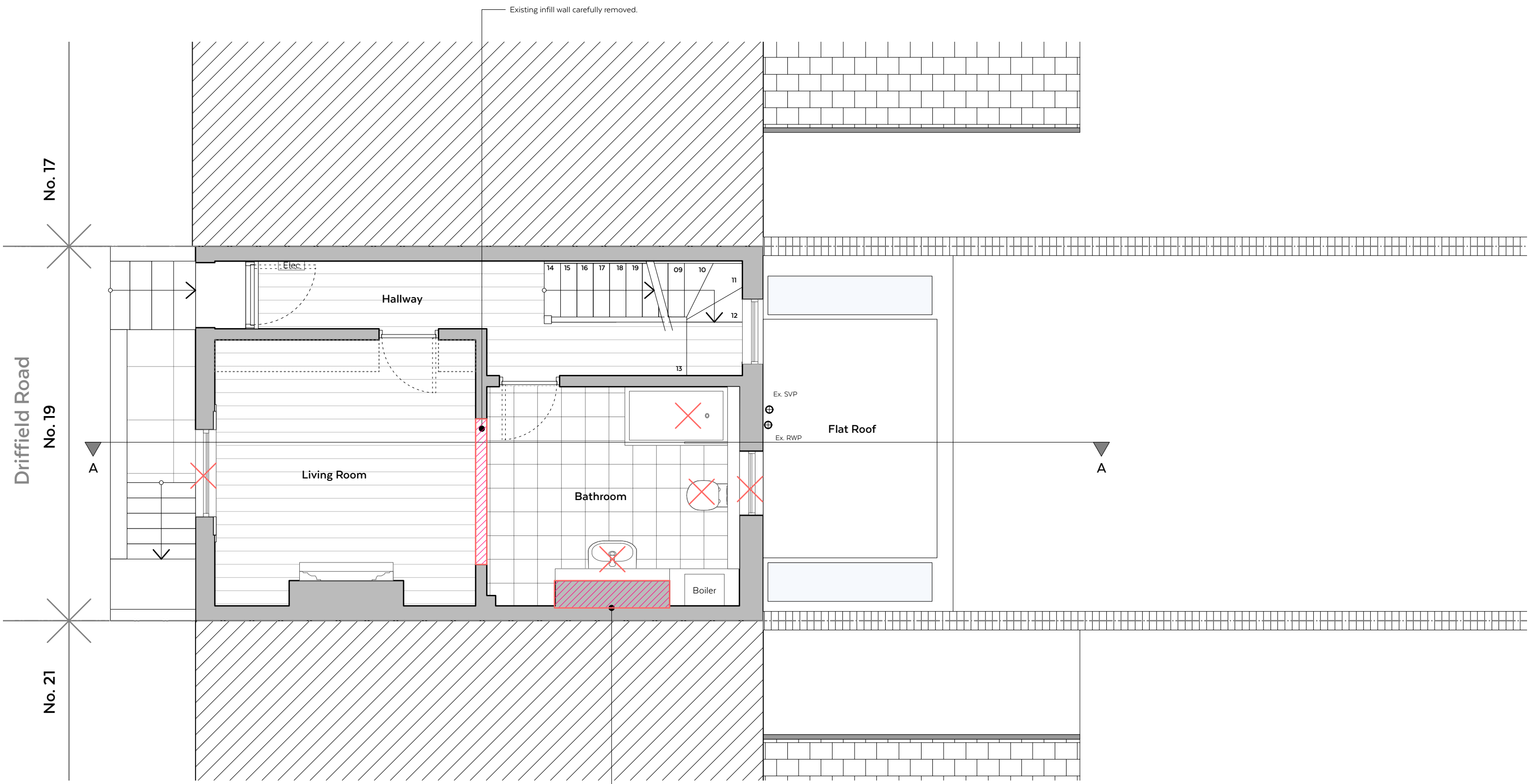
Existing Upper Ground Floor Plan - 1:50 @ A3
