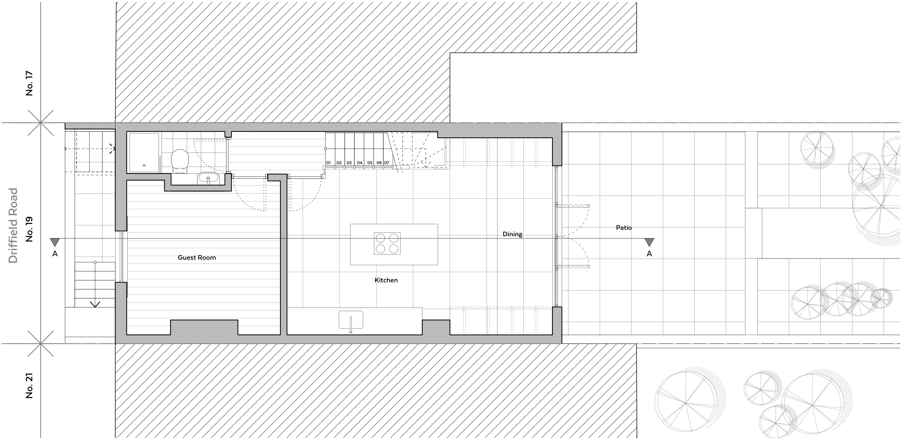
Proposed Lower Ground Floor Plan - 1:50 @ A3
