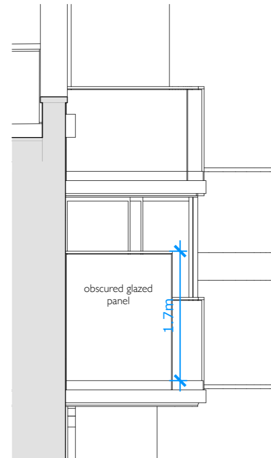
WEST ELEVATION
