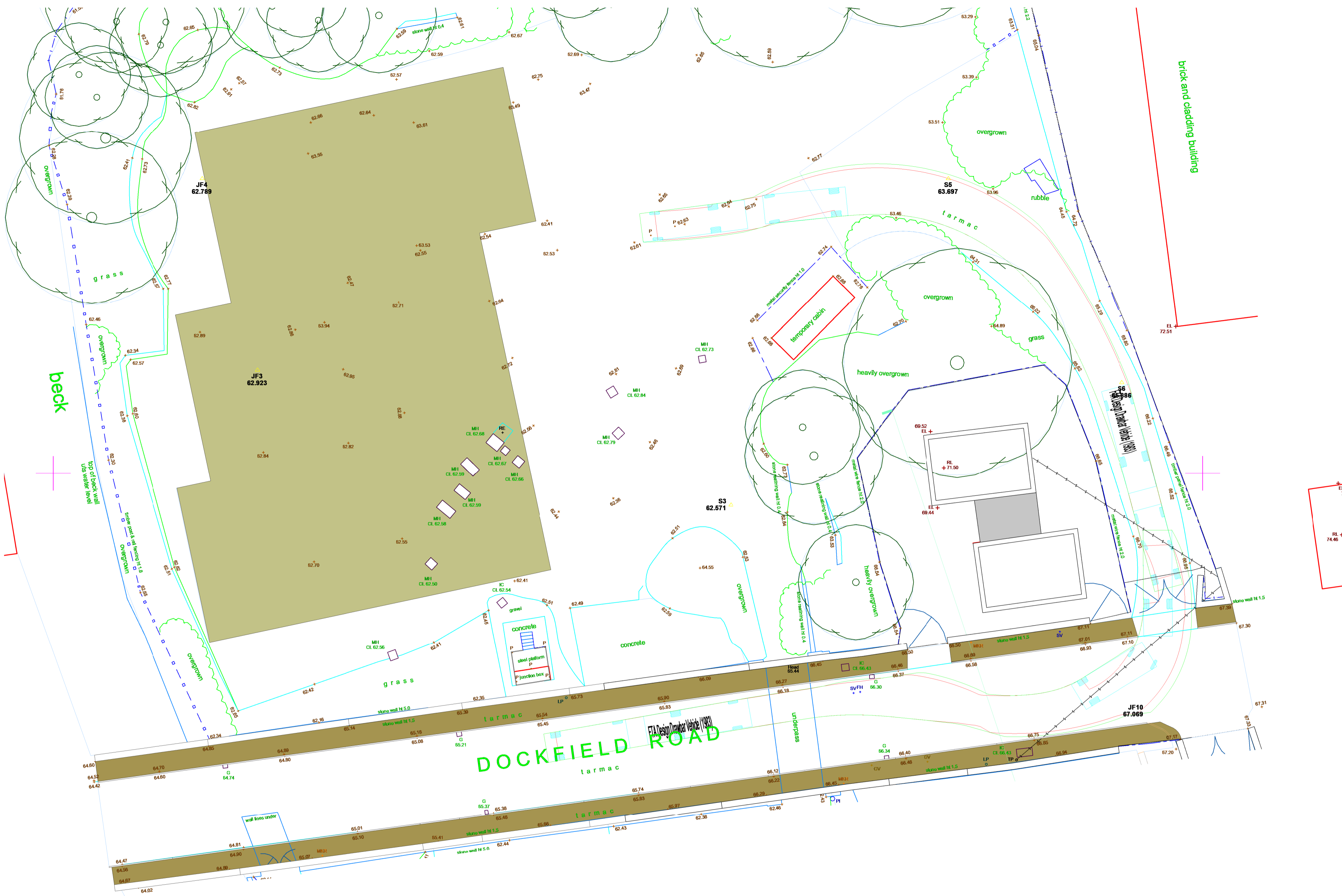
Vehicle Access North 1 : 200
