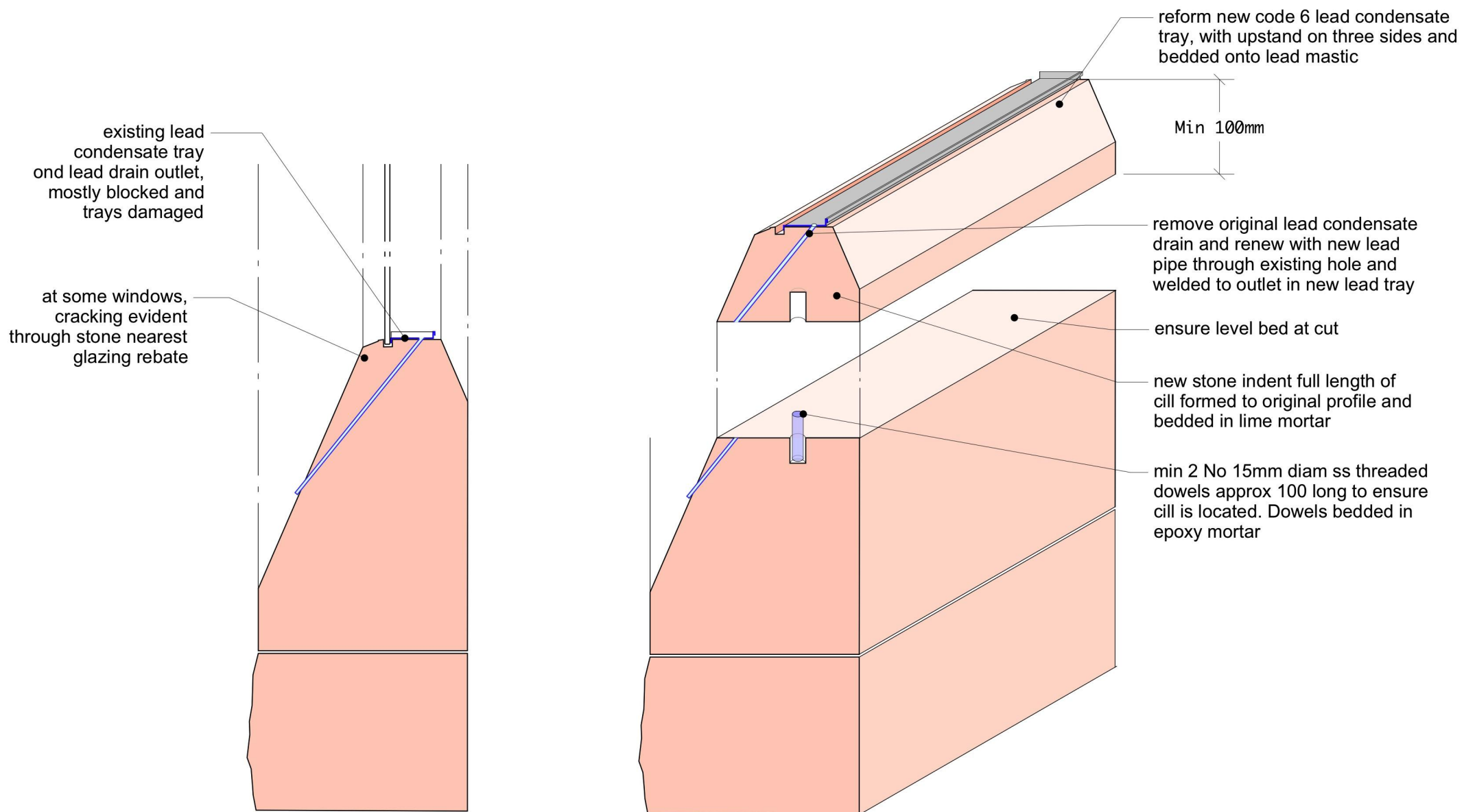
A) SECTION AT TYPICAL WINDOW
