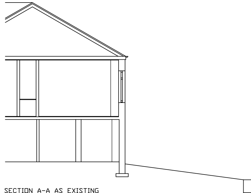
SECTION A-A AS EXISTING
