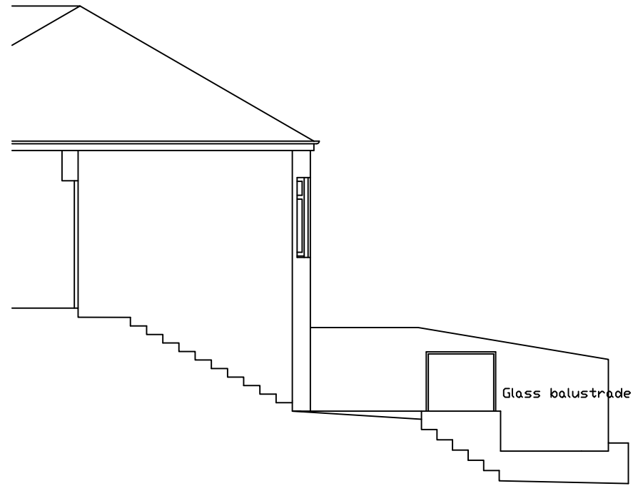
GABLE ELEVATION AS PROPOSED
