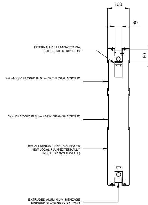
06 PROJECTING SIGN DETAIL P143059213 1:10@A3
