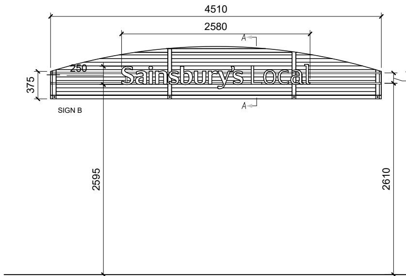
03 PROPOSED FASCIA SIGNAGE B - INTERNALLY ILLUMINATED - ILLUMINATION LEVEL - 375 cd/m 2 P143059213 1:50@A3
