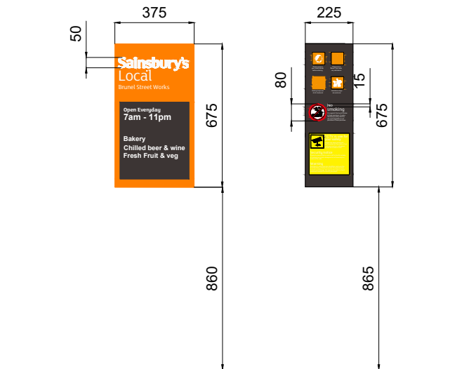
07 WELCOME MESSAGE P143059213 1:25@A3 08 STAT SIGN P143059213 1:25@A3
