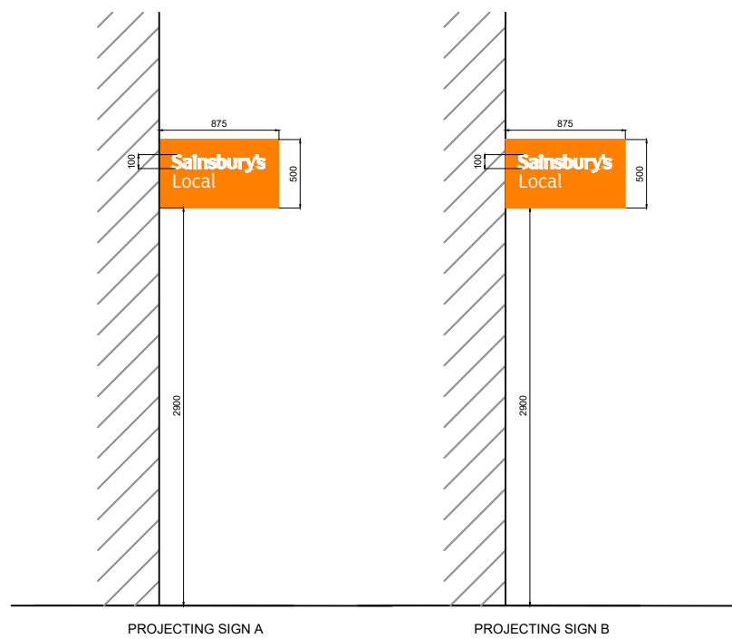
05 PROJECTING SIGNS P143059213 1:50@A3 ILLUMINATION LEVEL - 204 cd/m 2
