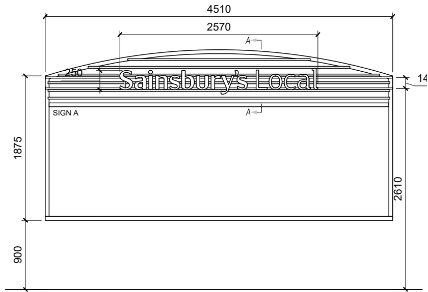
01 PROPOSED FASCIA SIGNAGE A - INTERNALLY ILLUMINATED - ILLUMINATION LEVEL - 375 cd/m 2 P143059213 1:50@A3
