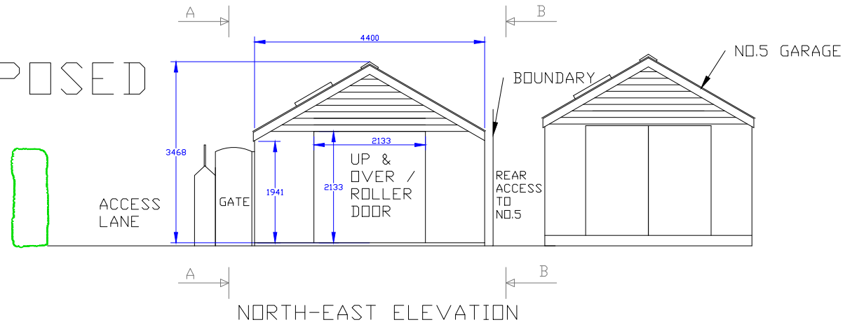
NORTH-EAST ELEVATION
