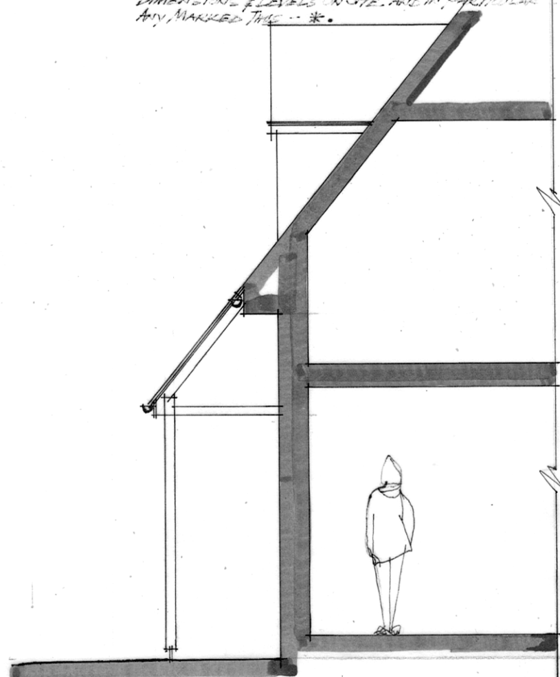
SIDE ELEVATION & SECTION - SOUTH WEST.
