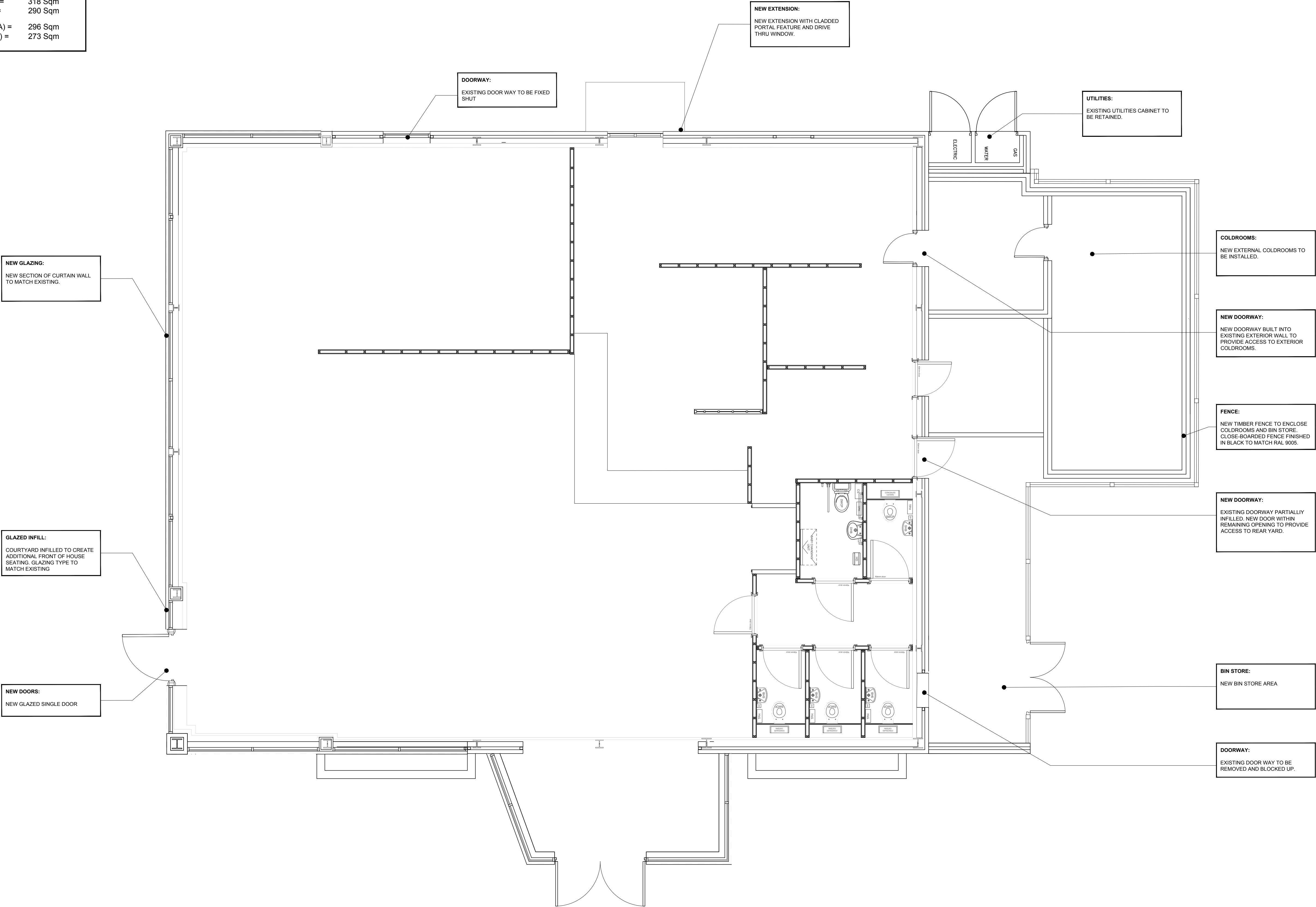
P PLAN PROPOSED GA PLAN SCALE 1:50 @ A1
