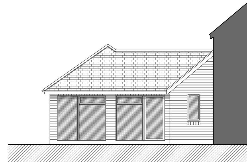
proposed drawing FRONT ELEVATION
