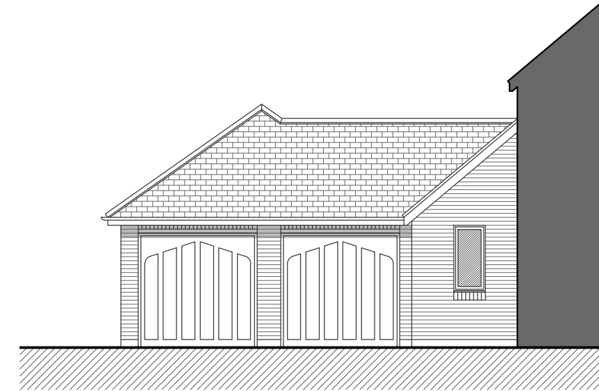
existing drawing FRONT ELEVATION
