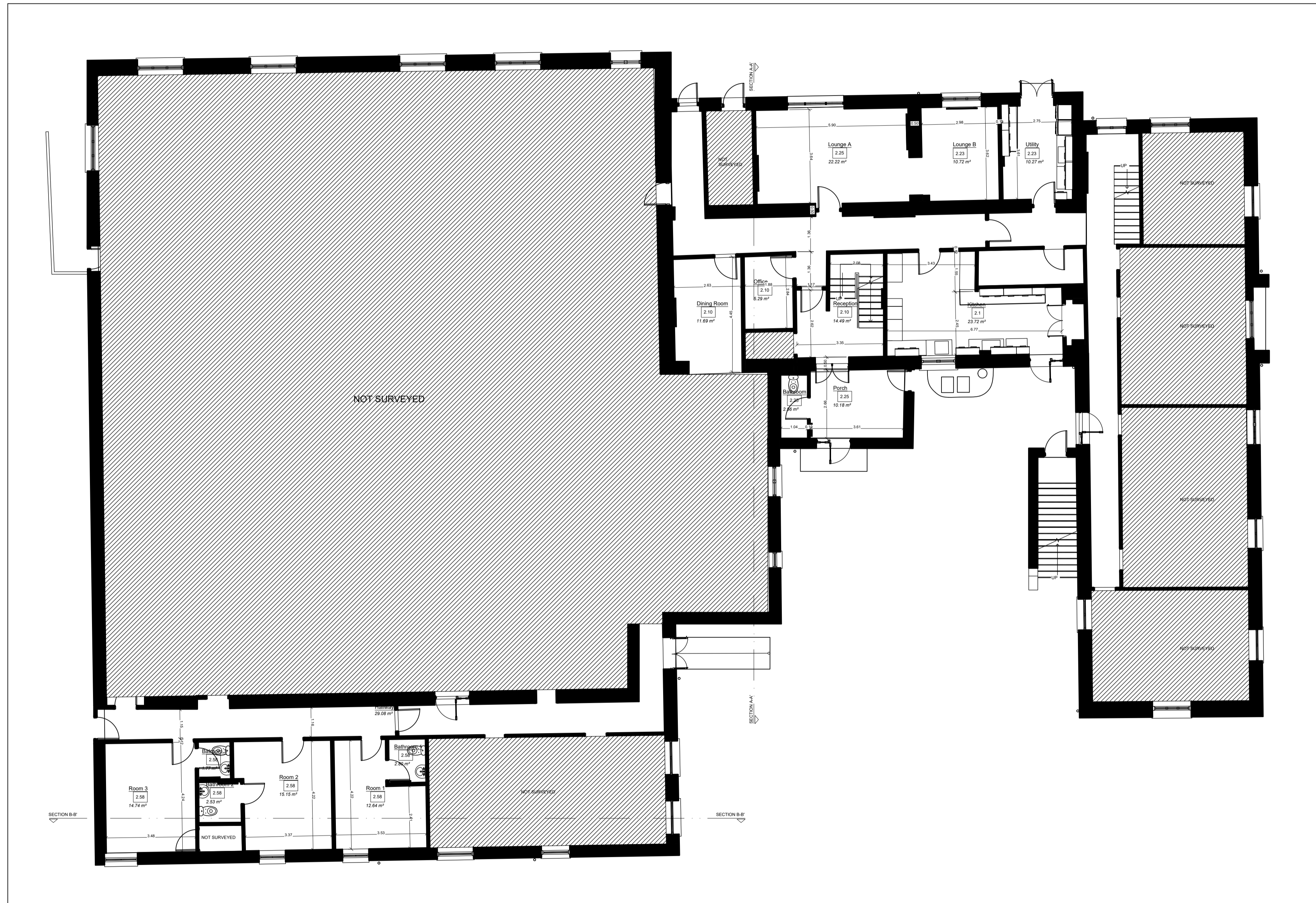
GROUND FLOOR 1/100
