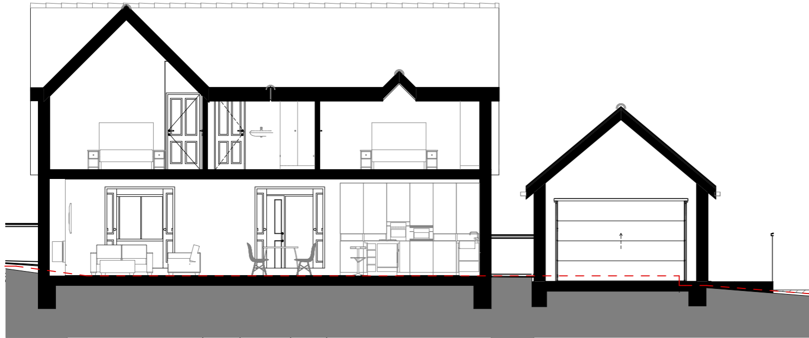
Section B-B
