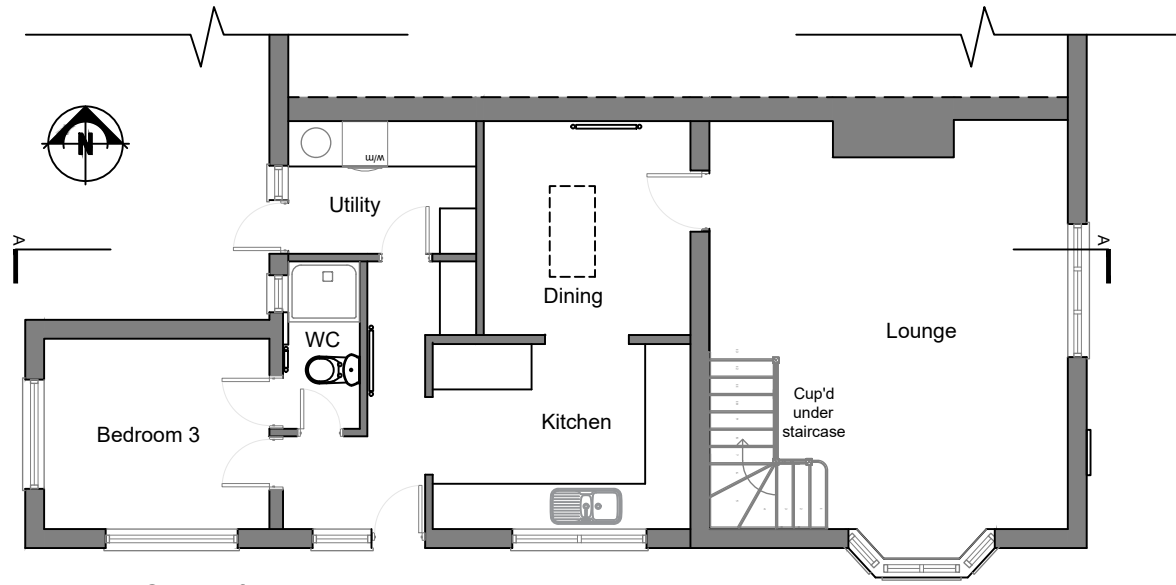
Ground floor 1:100
