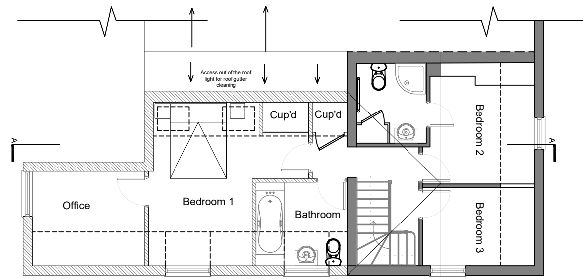
First floor 1:100
