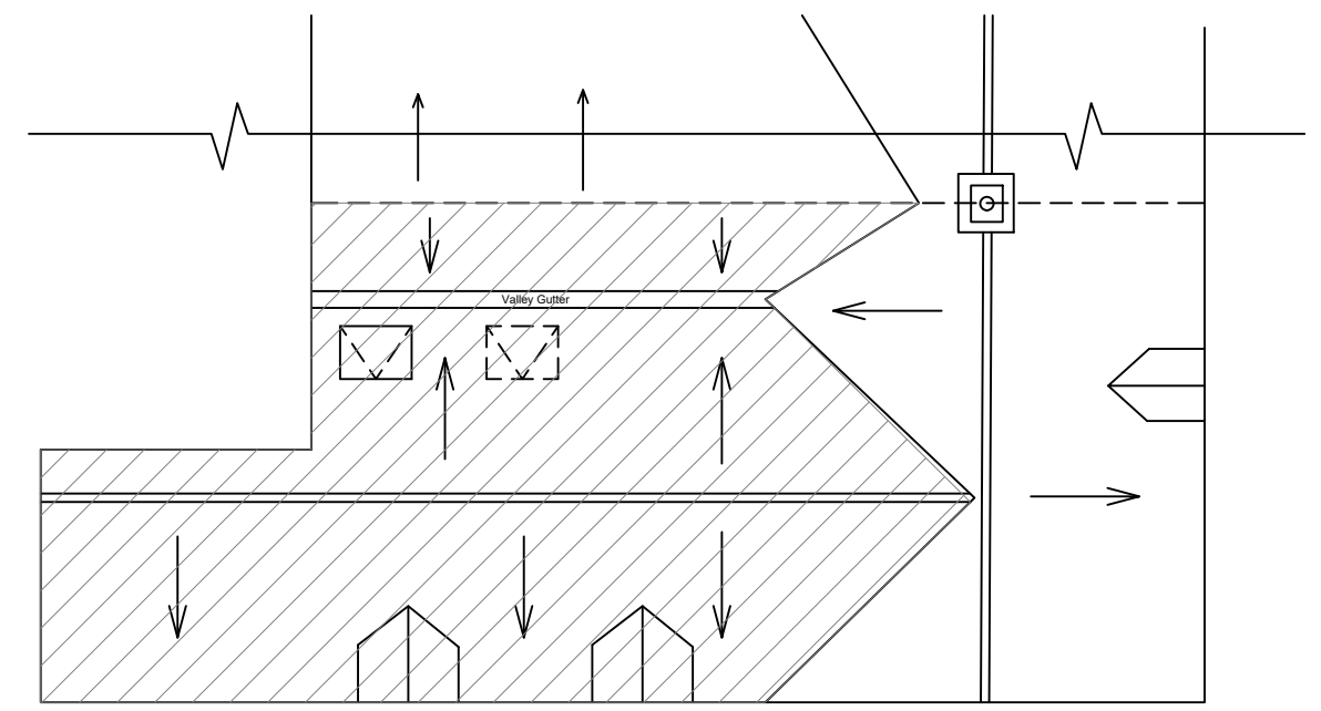
Roof plan 1:100
