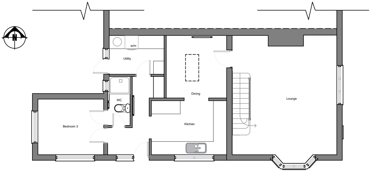
Ground floor 1:100
