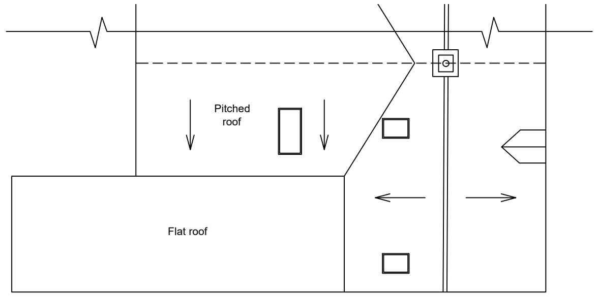
Roof plan 1:100
