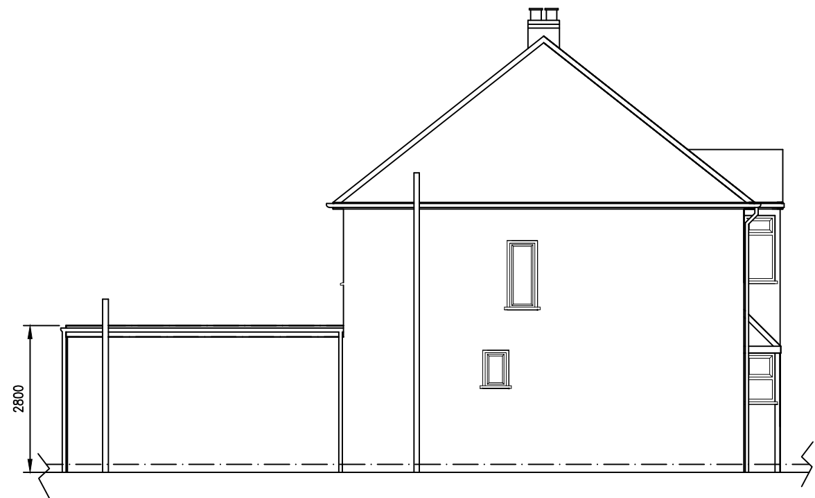
PROPOSED SIDE ELEVATION (viewed from No. 42)
