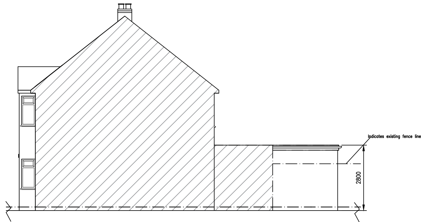
PROPOSED SIDE ELEVATION (viewed from No. 38)
