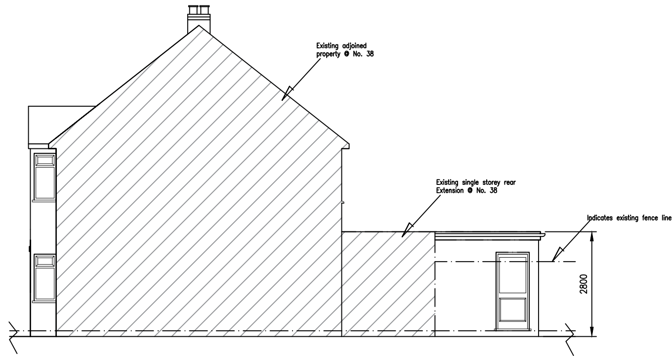
EXISTING SIDE ELEVATION (viewed from No. 38)
