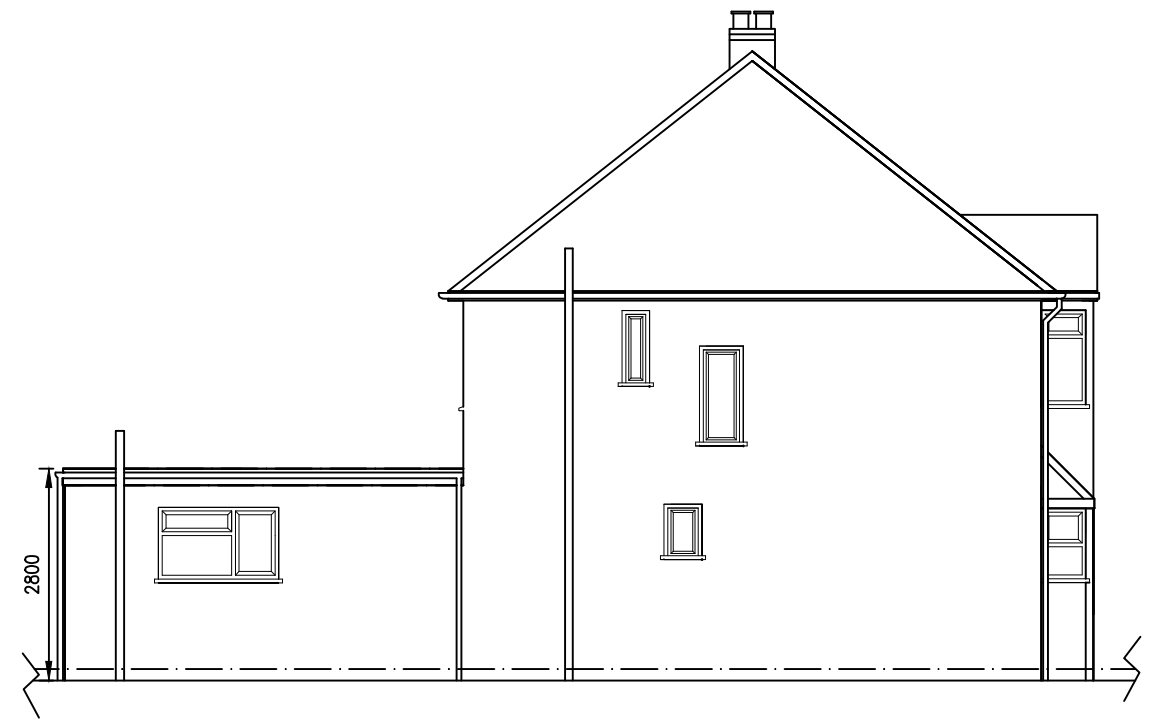
EXISTING SIDE ELEVATION (viewed from No. 42)
