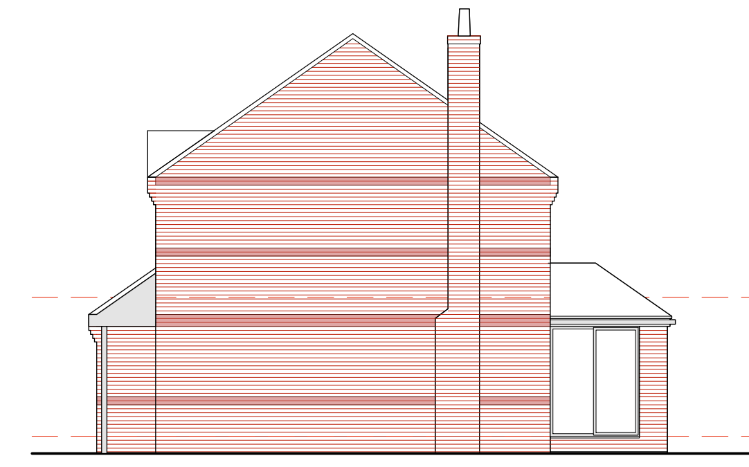
East Elevation 1:100
