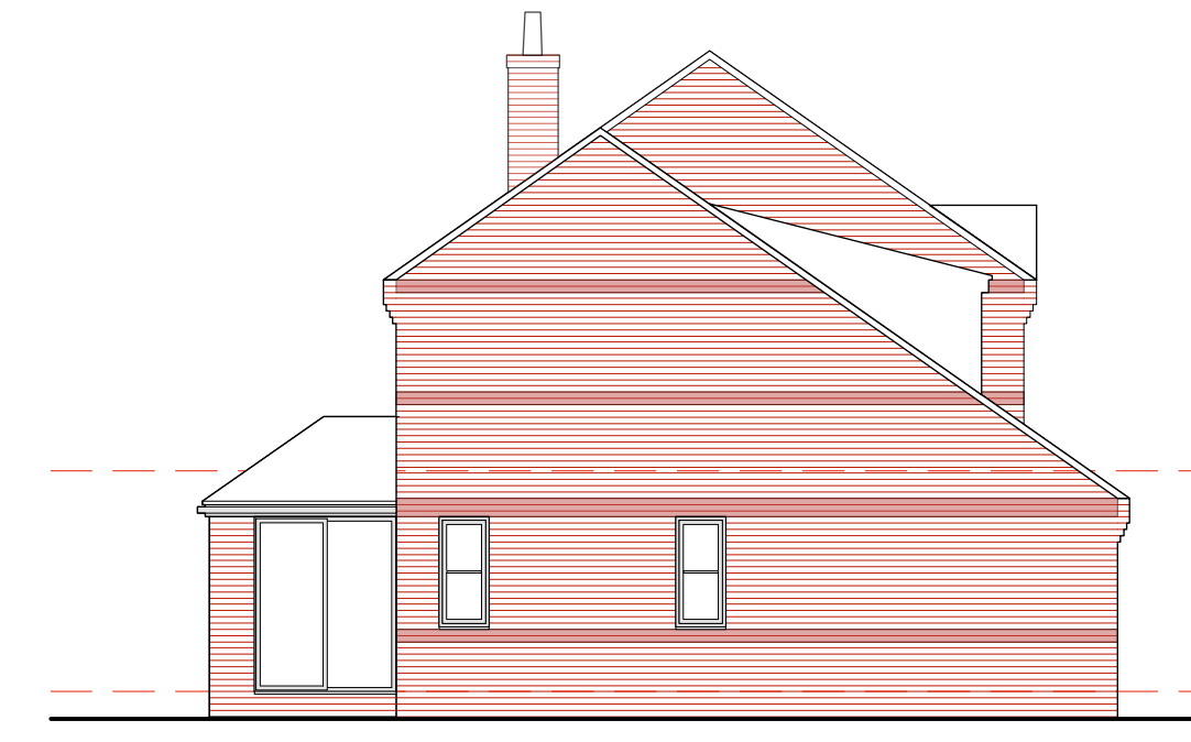
West Elevation 1:100
