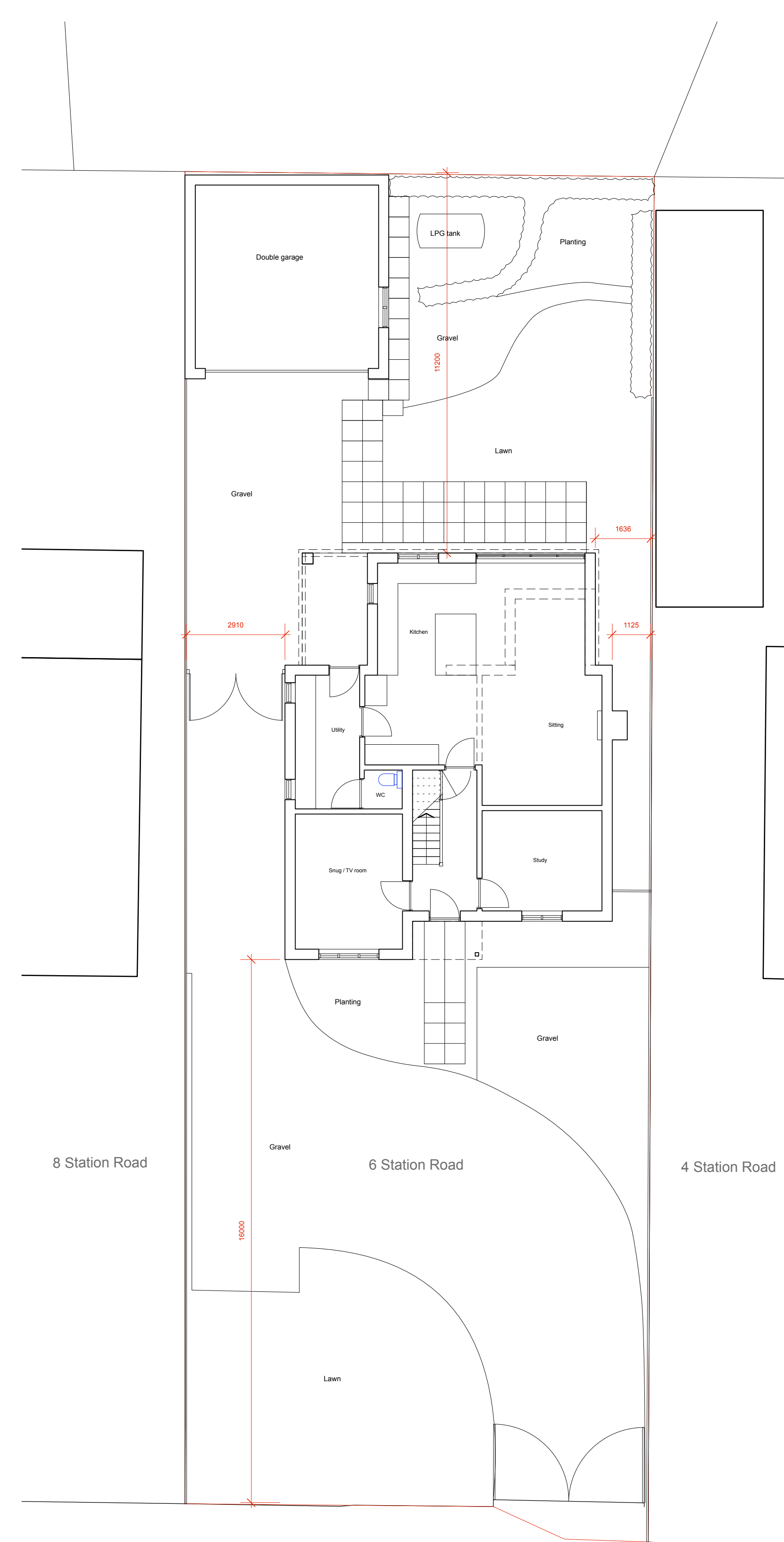
Site and Ground floor plan 1:100
