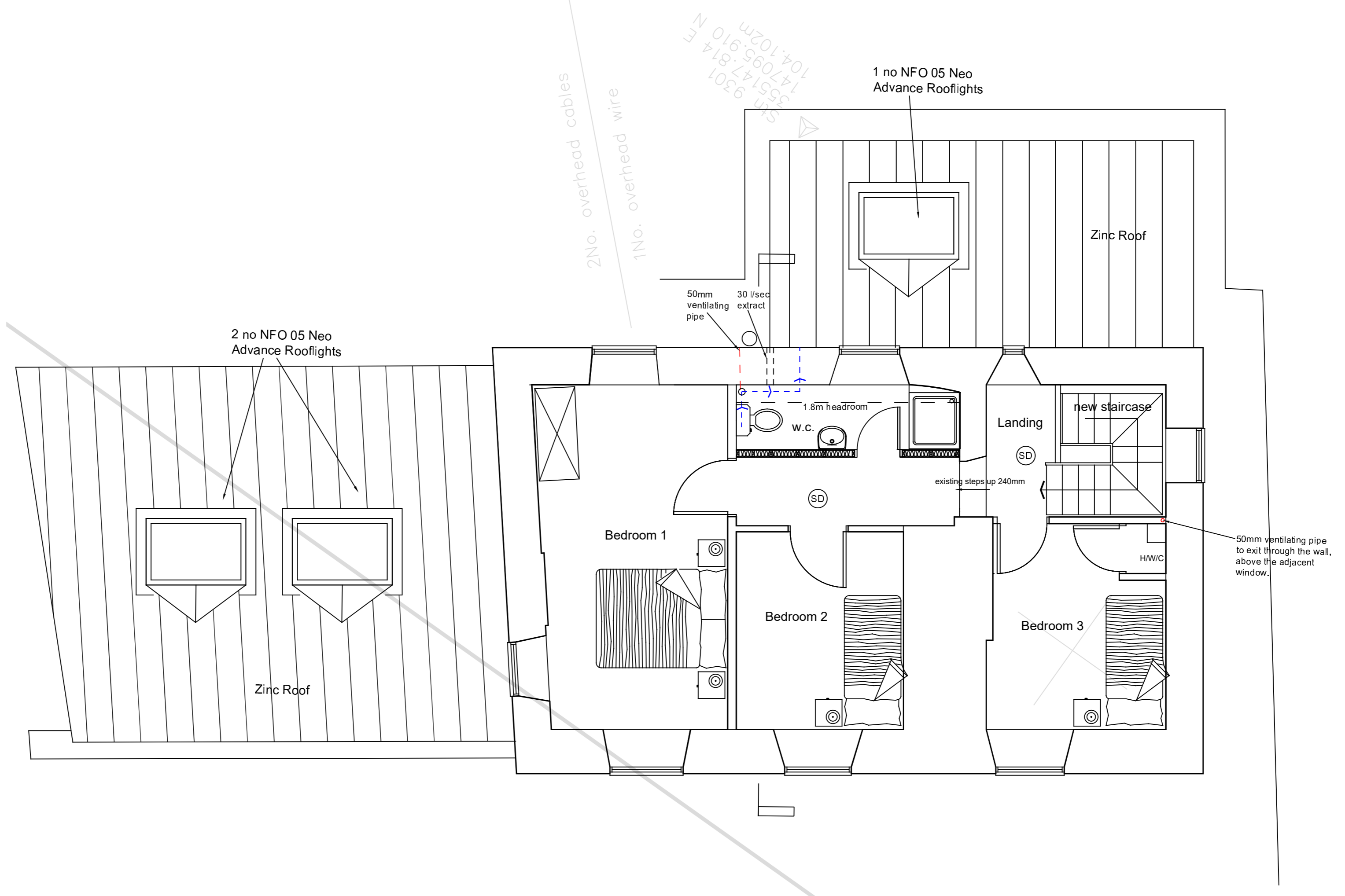
FIRST FLOOR
