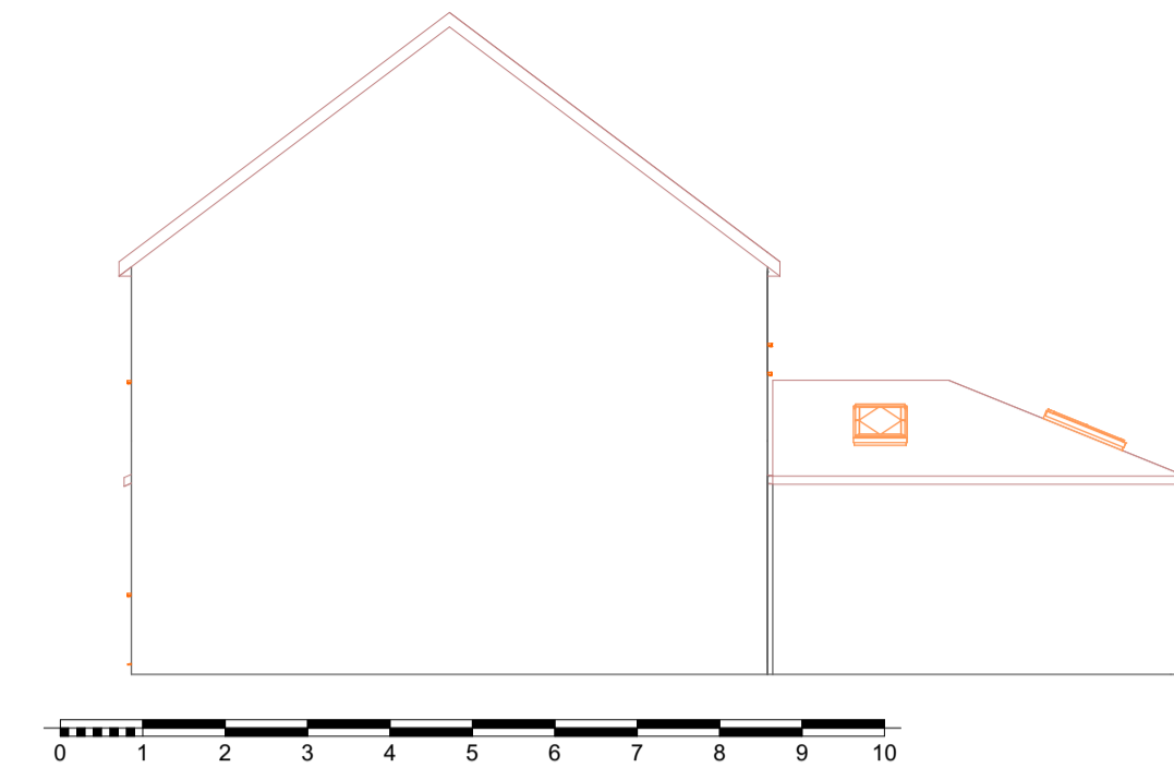
5 East Elevation Proposed 1:100
