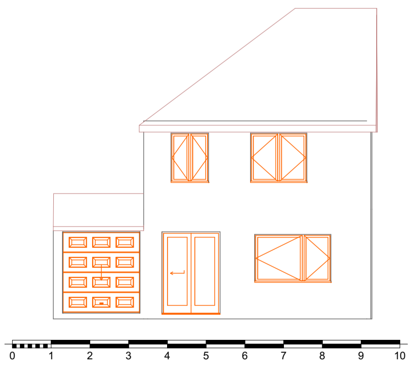
4 South Elevation Existing 1:100
