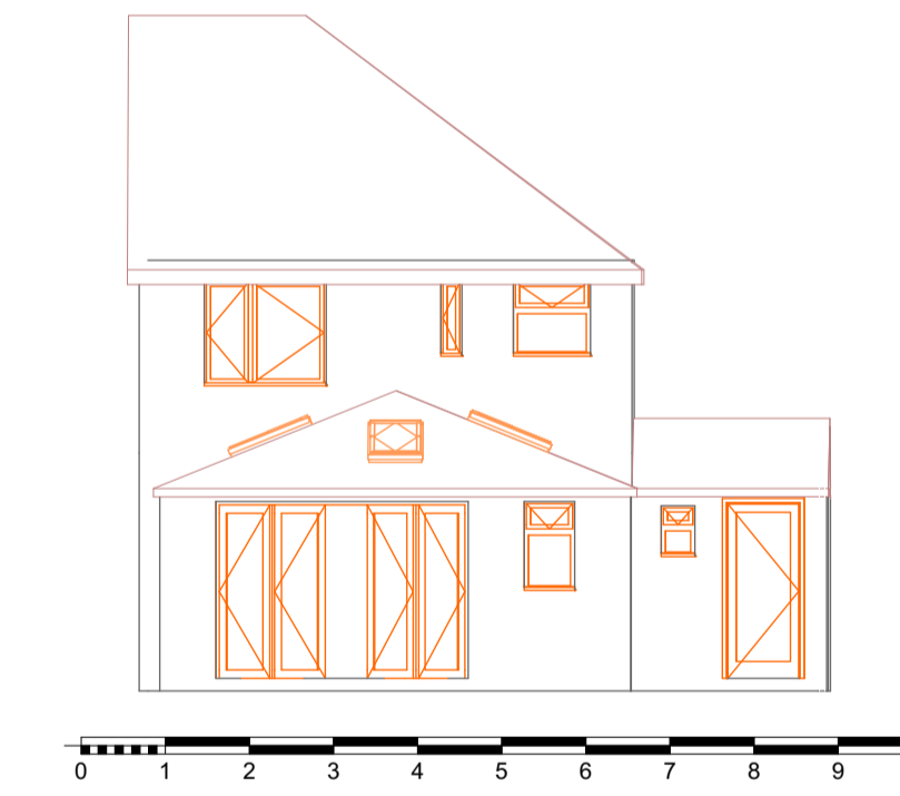
6 West Elevation Proposed 1:100
