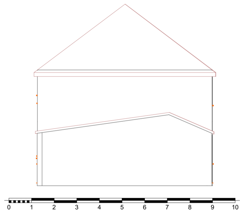
2 West Elevation Existing 1:100
