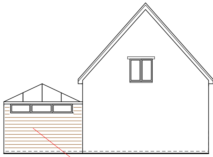
rear (north) elevation
