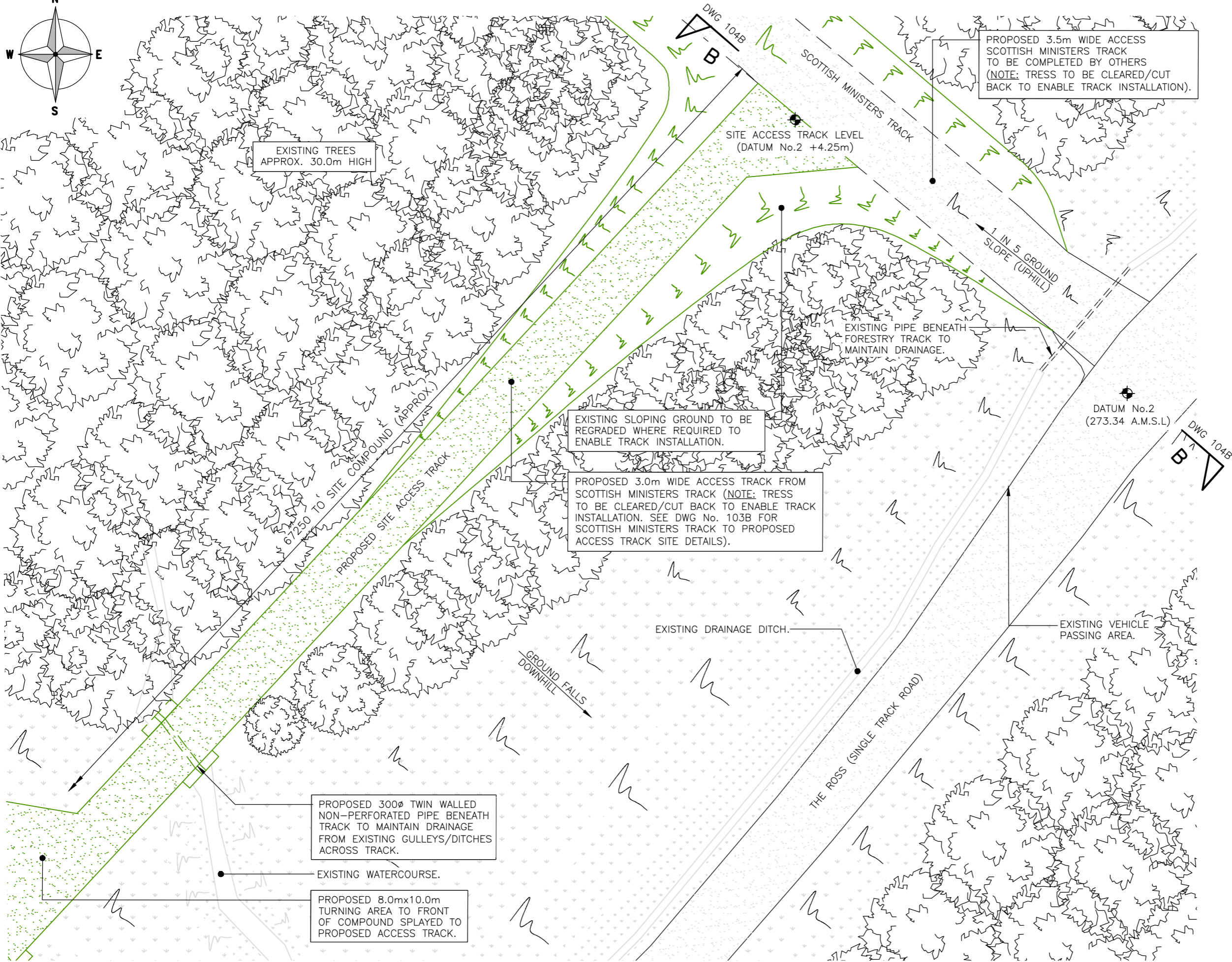
PROPOSED SITE ENTRANCE PLAN (1:200)
